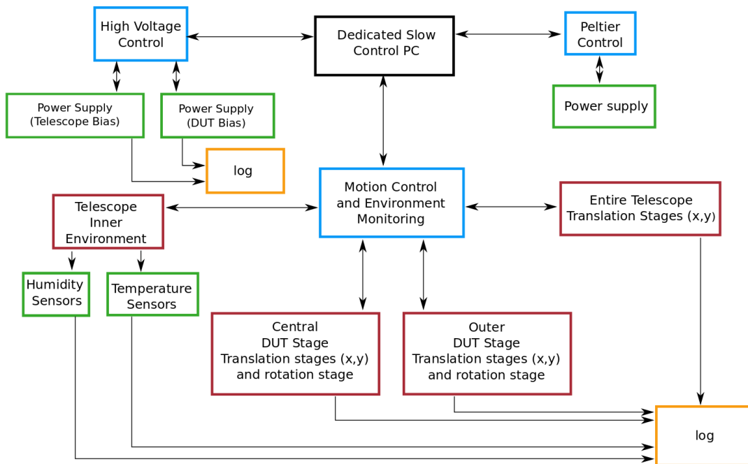
Figure 2: Block diagram of the slow control system. The telescope and DUT bias voltages and motion stages are operated remotely. The bias currents and temperatures of the telescope environment are monitored and logged.
