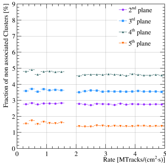
Figure 7: Fraction of clusters not associated to a reconstructed track in the internal planes of the telescope. In the high-rate configuration the telescope was constituted by 6 planes only. The plane-to-plane variation does not depend on the rate and remains constant. This is attributed to slight differences among the ASICs.
