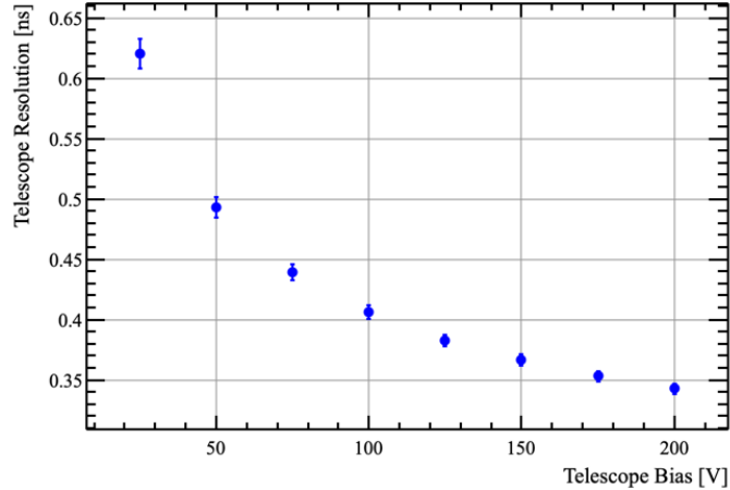
Figure 4: Resolution of track timestamps as function of bias voltage, using eight telescope planes.
