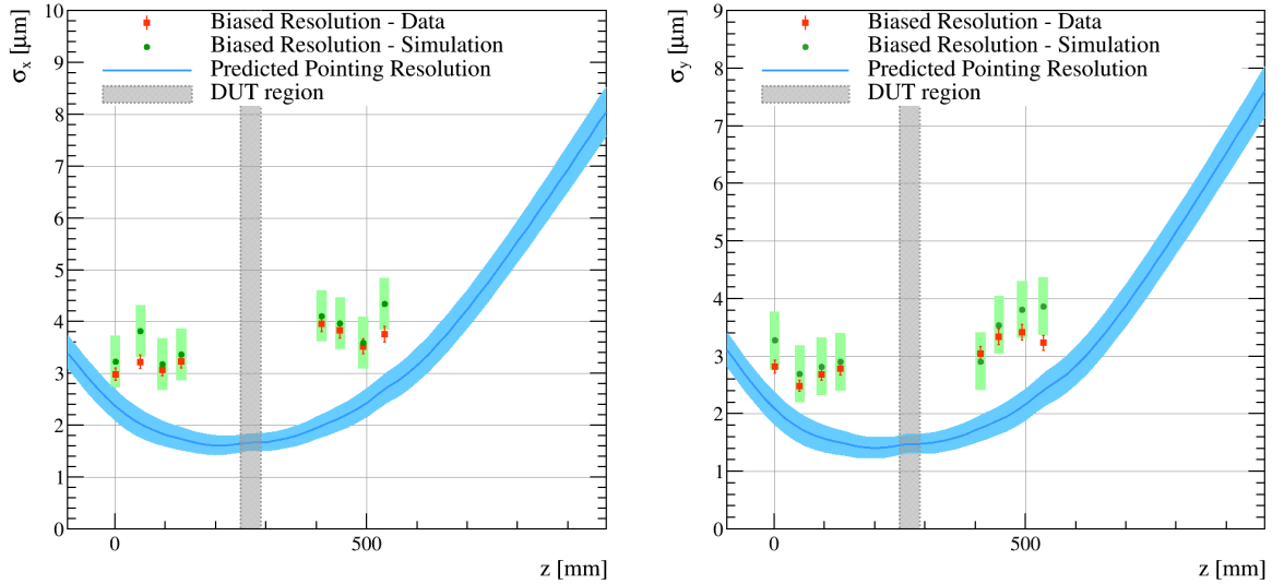
Figure 6: Predicted pointing resolution and uncertainty (solid blue curves) in the x coordinate (left plot) and y coordinate (right plot). The green dots show the Monte Carlo biased resolution and the applied uncertainty is indicated by green bars. The red points show the biased resolution measured in the data. The typical installation position for a DUT is illustrated by the hatched grey region.
