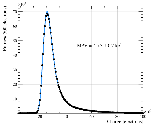
Figure 3: Typical distribution of collected charge of associated clusters for a telescope plane. The curve shows the Landau convoluted with a Gaussian fit.
