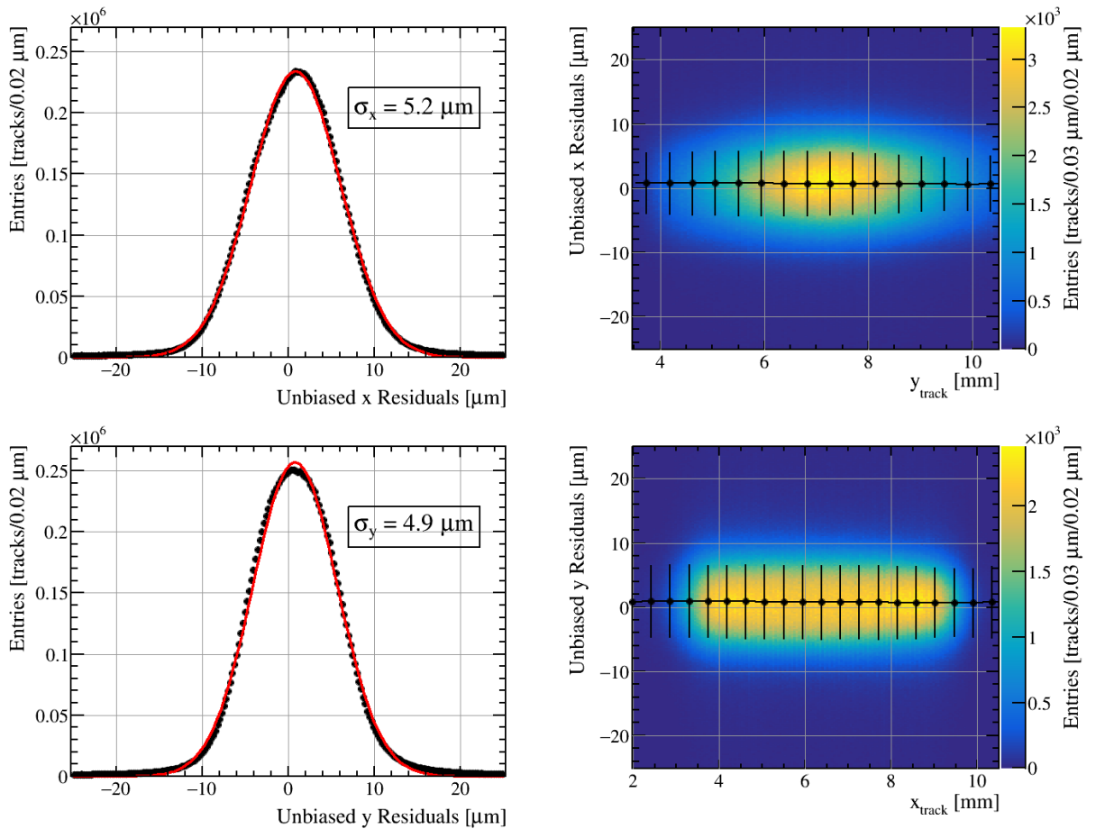
Figure 5: Unbiased residuals in x and y on one telescope plane, both integrated over the chip and as a function of position. The error bars show the fitted gaussian width at each position.
