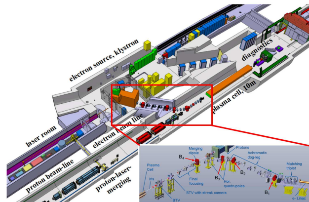
Figure 1: AWAKE tunnel and current electron beamline.
