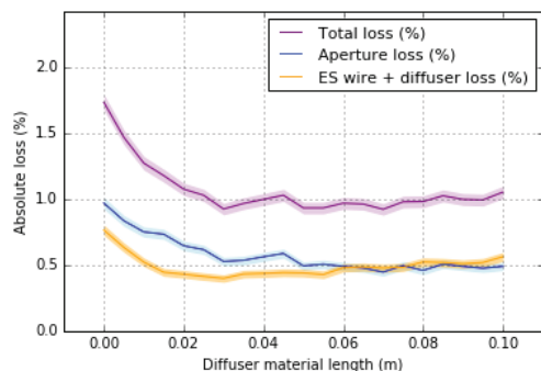
Figure 3: 8 GeV loss vs. length for 0.2 mm wide C diffuser and 0.2 mm W/Re ES.
