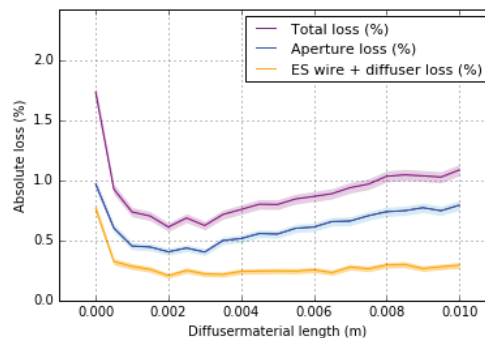
Figure 1: 8 GeV loss vs. length for 0.2 \text{ mm} wide Ta diffuser 1^\circ upstream of 0.2 \text{ mm} W/Re ES.
