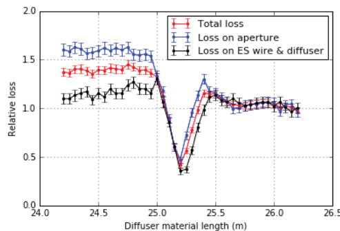
Figure 2: 8 GeV loss vs. position for 2 \text{ mm} long, 0.2 \text{ mm} wide Ta diffuser 1^\circ upstream of 0.2 \text{ mm} wide W/Re ES.
