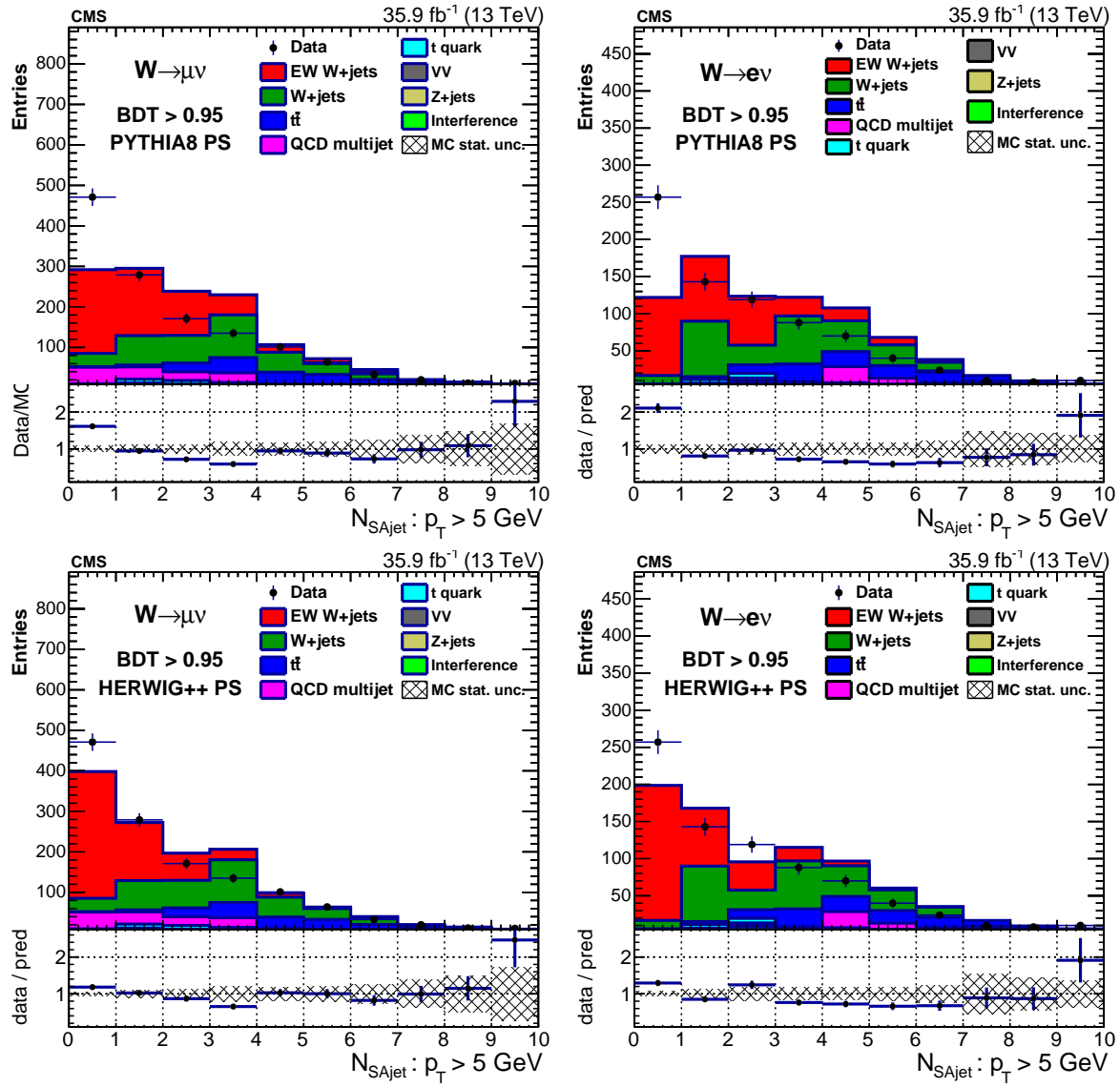
Figure 21: Number of soft activity jets with p_T > 5 GeV in the rapidity gap for BDT > 0.95 in the muon (left) and electron (right) channels including signal with PYTHIA parton showering (upper) and HERWIG++ parton showering (lower).
