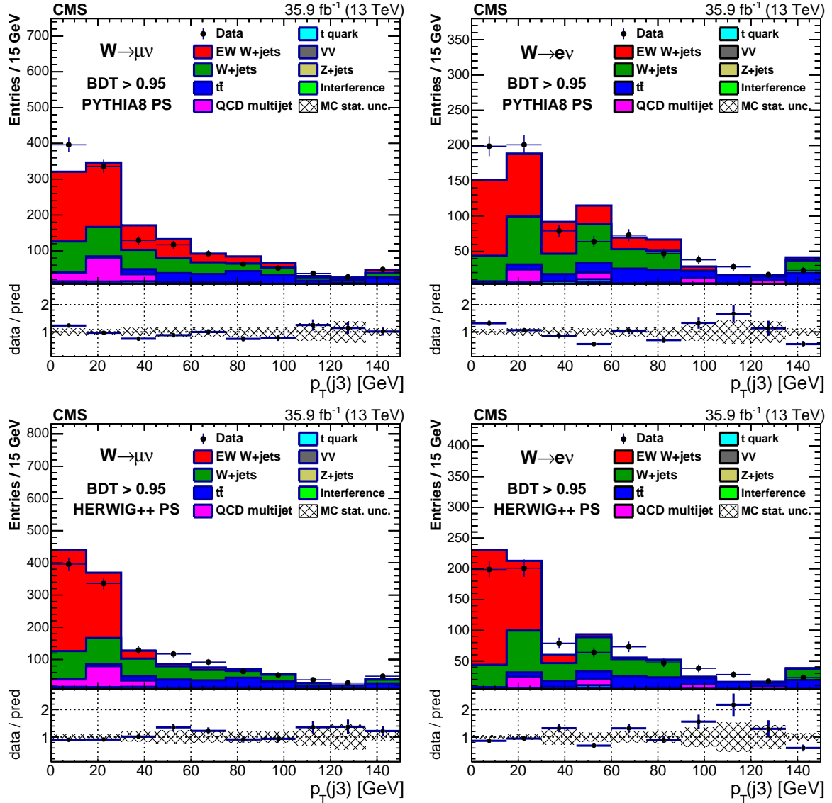
Figure 15: Leading additional jet p_T ( p_T(j_3) ) for \text{BDT} > 0.95 in the muon (left) and electron (right) channels including the signal prediction from MADGRAPH5_aMC@NLO interfaced with PYTHIA parton showering (upper) and HERWIG++ parton showering (lower). In all plots the last bin contains overflow events, and the first bin contains events where no additional jet with p_T > 15 \text{ GeV} is present.
