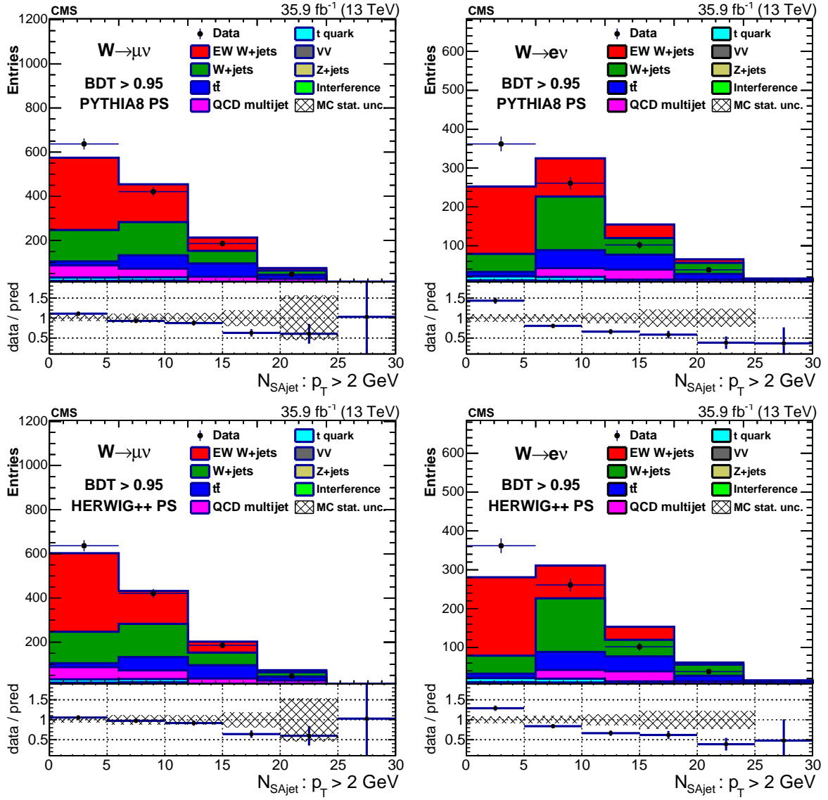
Figure 22: Number of soft activity jets with p_T > 2 \text{ GeV} in the rapidity gap for \text{BDT} > 0.95 in the muon (left) and electron (right) channels including signal with PYTHIA parton showering (upper) and HERWIG++ parton showering (lower).
