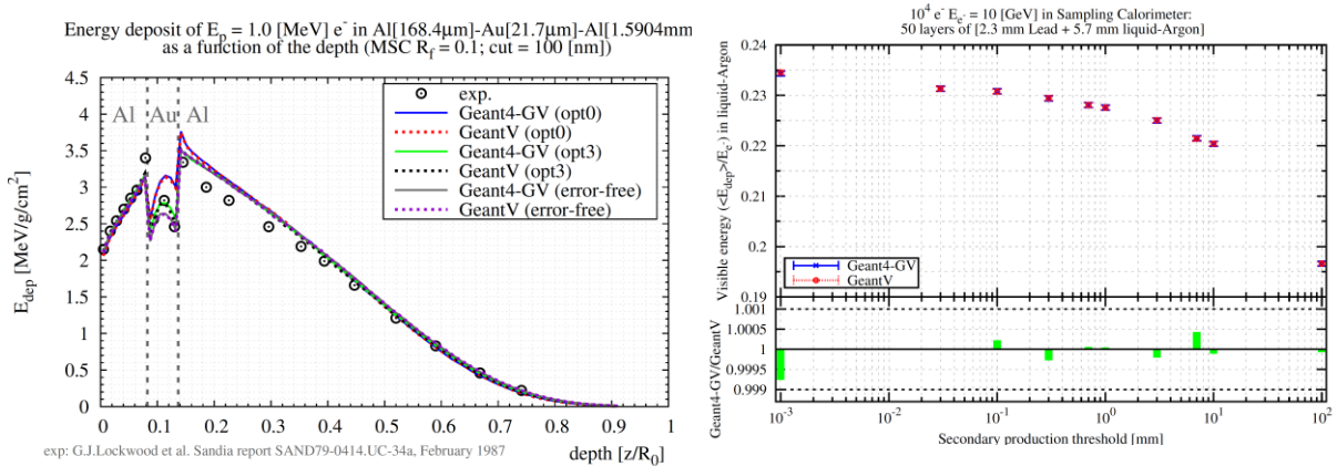
Figure 5 GeantV EM physics validation against Geant4 10.4 beta. Left: Energy deposit depending on depth for 1 MeV electrons in multi-layered Al-Au-Al target. Different options of the multiple scattering model have been compared for GeantV, Geant4 and data. Right: visible energy per primary for 10 GeV electrons in liquid-Argon for multi-layered sampling calorimeter. The Geant4-GV physics list matching the physics settings used in GeantV was consistently used in Geant4-based simulations.
