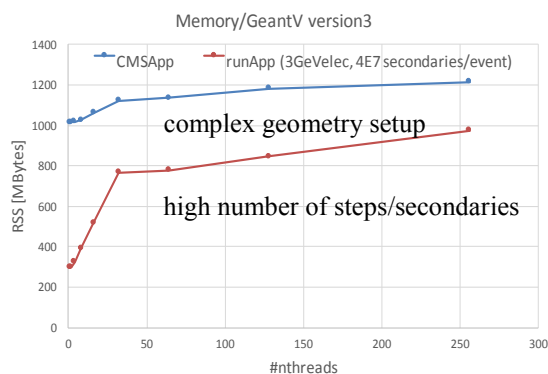
Figure 2 Resident Set Size (RSS) vs number of threads. Memory in GeantV scheduler (version 3) is controlled by applying a policy prioritizing the transport of older generation secondary particles, while re-using the containers released by completed tracks.
