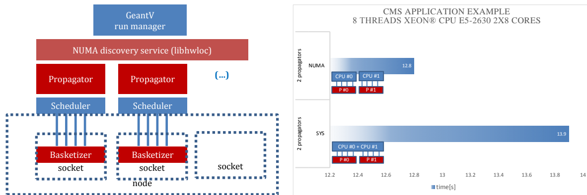
Figure 4 Left: schematic mapping of GeantV track transport services to machine topology. Right: Benefits of deployment of a number of propagators matching the number of locality nodes (sockets) of the machine. The alpha release of GeantV can be configured NUMA-aware, detecting the hardware topology and confining the data and processing flow to local resources as much as possible.
