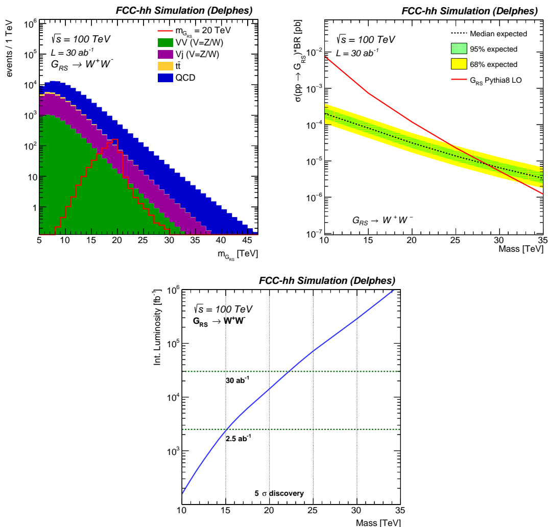
Fig. 9. Invariant mass distribution of the two selected W-jets for a 20 TeV signal (left), 95% CL limit versus mass (right) and 5\sigma discovery reach (bottom).
