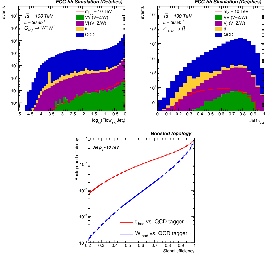
Fig. 15. Left: Energy-flow E_F(n = 1, \alpha = 0.05) observable for the leading jet p_T of the G_{RS} \rightarrow W^+W^- analysis at the pre-selection level (two high p_T jets). Right: \tau_{32} observable for the leading jet p_T of the Z' \rightarrow t\bar{t} analysis at the pre-selection level (two high p_T jets). Bottom: Light jet rejection versus tagging efficiency for the W -tagger (blue) and top-tagger (red)
