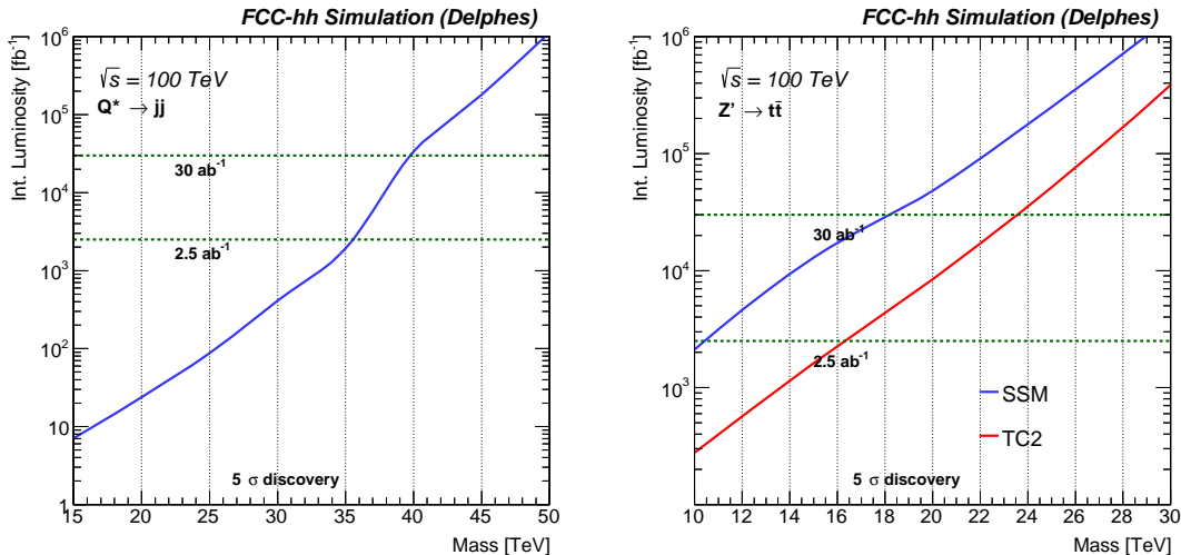
Fig. 8. 5\sigma discovery reach for the jj (left) and t\bar{t} (right) final states.
