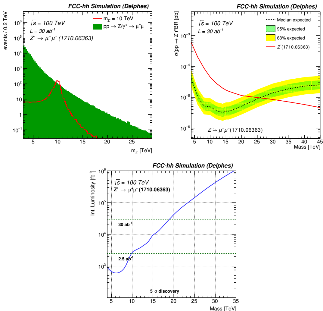
Fig. 5. Left : Invariant mass for a 10 TeV signal after full event selection in flavour anomaly scenario. Limit versus mass (right) and luminosity for a 5\sigma discovery (bottom).
