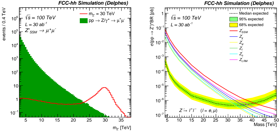
Fig. 2. Left: Invariant mass for a 30 TeV signal after full event selection for the \mu\mu channel. Right: 95% CL limit versus mass for the combined di-lepton ( ee, \mu\mu ) channel.
