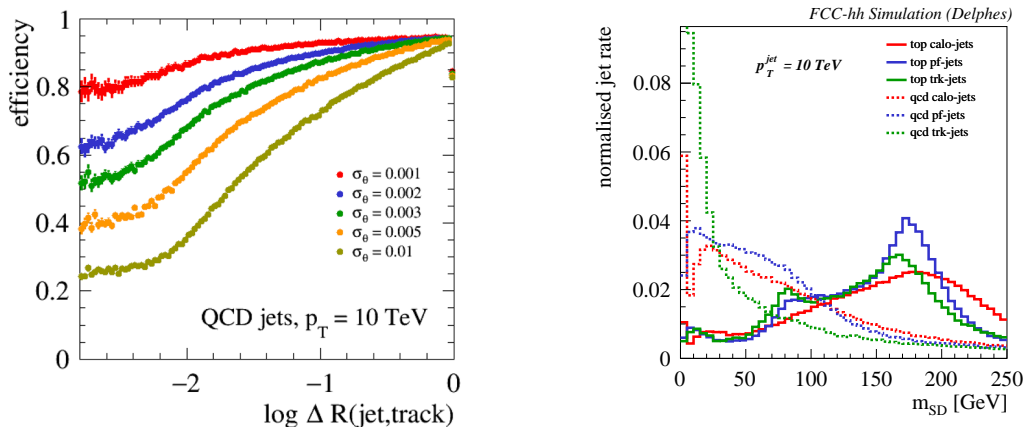
Fig. 1. Left: Track reconstruction efficiency inside highly boosted QCD jets as function of the angular distance \Delta R between the track and the center of the jet for different assumptions on the tracker spatial resolution. Right: Reconstructed "soft-dropped" jet mass of highly boosted top and QCD jets with various sets of input to the jet clustering algorithm: tracks only, calorimeters towers only and particle-flow candidates.
