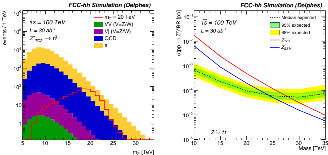
Fig. 7. Invariant mass distribution of the two selected top-jets (left) for a 20 TeV signal (left), 95% CL limit versus mass (right).
