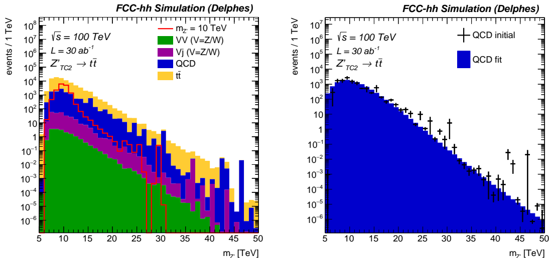
Fig. 14. QCD Background invariant mass spectra prior to fit.
