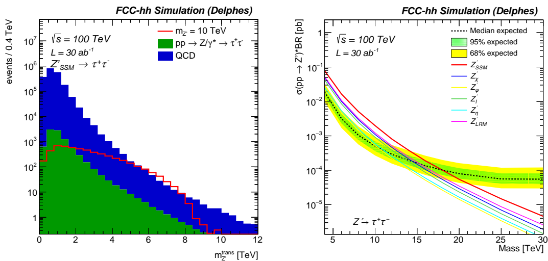
Fig. 3. Left: Di- \tau transverse mass for a 10 TeV signal after full event selection. Right: 95% CL limit versus mass.
