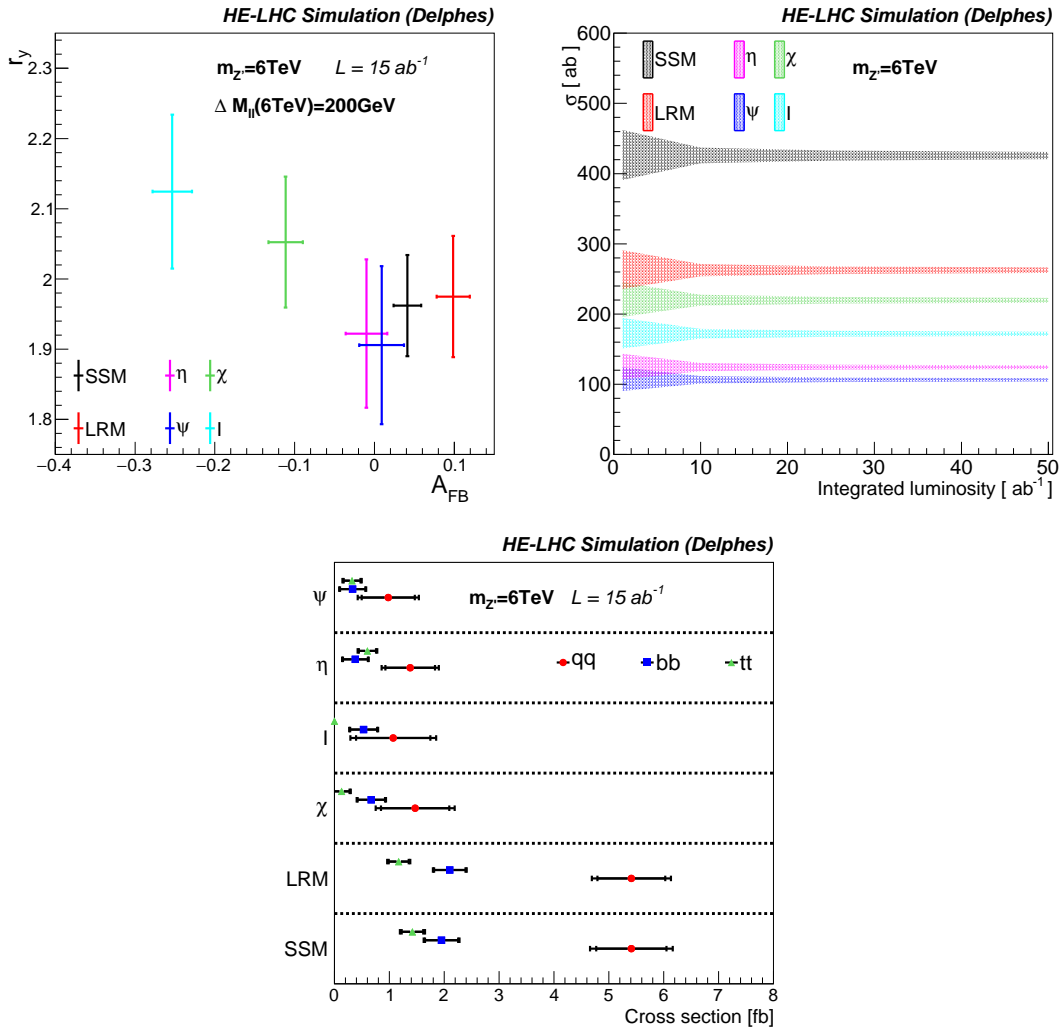
Fig. 12. Left: Scatter plot of r_y versus A_{FB} with a 200 GeV mass window. The full interference is included. Right: Fitted signal cross-section together with its corresponding error versus integrated luminosity. Bottom: Fitted cross-section of the three hadronic analyses. Statistical and full uncertainties are shown on each point.
