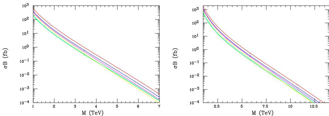
Fig. 11. Left: \sigma B_l in the NWA for the Z' production at the \sqrt{s} = 14 TeV LHC as functions of the Z' mass: SSM (red), LRM (blue), \psi (green), \chi (magenta), \eta (cyan), I (yellow). (Right) \sigma B_l of Z' in models described in (left) at \sqrt{s} = 27 TeV.
