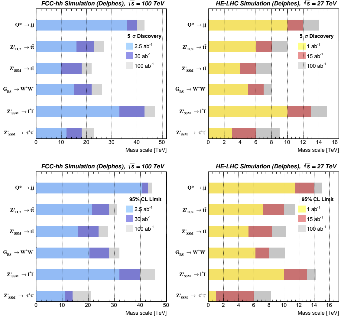
Fig. 16. Summary of a 5\sigma discovery reach (top) and 95% CL limits (bottom) as a function of the resonance mass for different luminosity scenario of FCC-hh (left) and HE-LHC (right).
