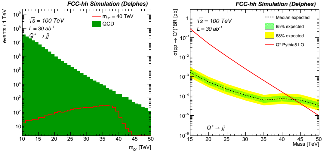
Fig. 6. Invariant mass distribution of the two selected jets for a 40 TeV signal (left), 95% CL limit versus mass (right).
