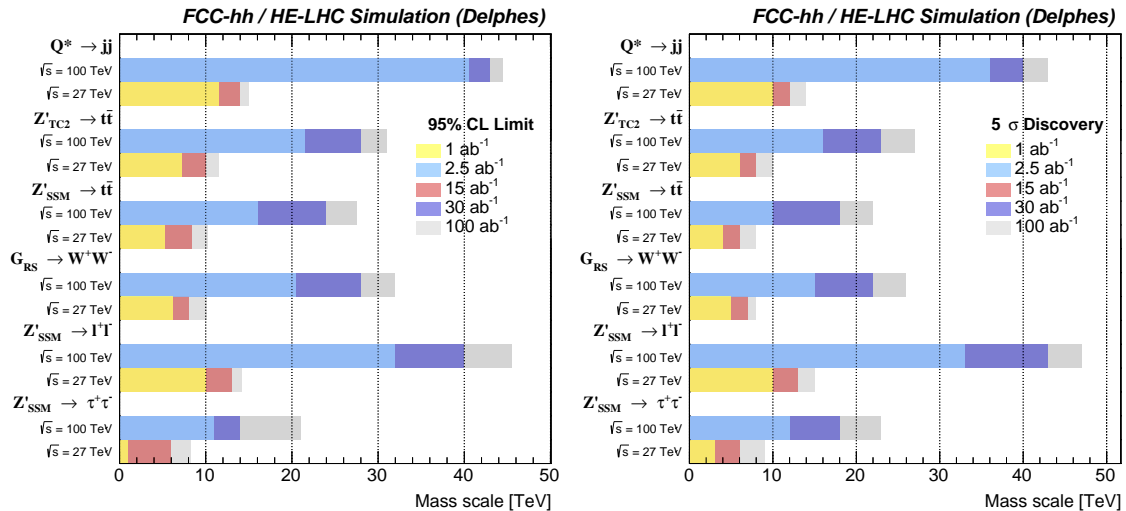
Fig. 10. Summary of the 95% CL limits (left) and 5\sigma discovery reach (right) as a function of the resonance mass for different luminosity scenario of FCC-hh and HE-LHC.
