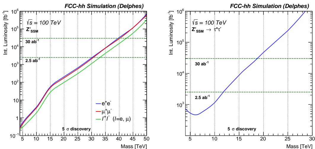
Fig. 4. Integrated luminosity versus mass for a 5\sigma discovery, for e/\mu final states (left) and for the \tau final states (right).
