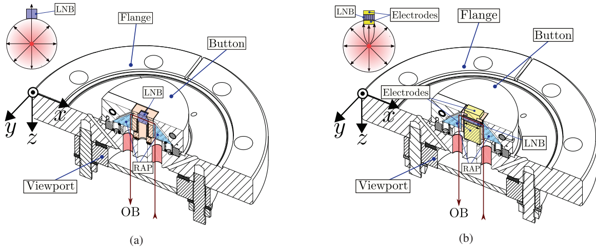
Figure 1: Prototyp pick-up variants: zero (a) with only a crystal; and one (b) with an additional electrode.
