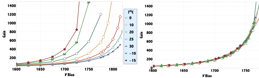
Figure 2: Left: Gain of a 8 \times 8 \text{ mm}^2 APDs as a function of bias voltage at different temperatures. The measurement was performed using a blue LED. Right: By shifting the bias for each curve according to the law described in the text, a scaling law is found.
