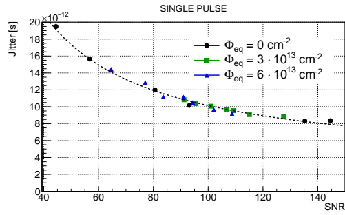
Figure 12: Single pulse time resolution of the 2 \times 2 \text{ mm}^2 APDs as a function of signal to noise ratio and fluence measured at -20^\circ\text{C} . The laser intensity corresponds to 0.8 MIPs. An amplification of 40 dB was used.
