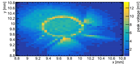
(e) \Phi_{eq} = 10^{15} \text{ cm}^{-2} , 1644 V
