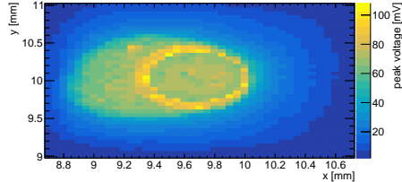
(c) \Phi_{eq} = 6 \cdot 10^{13} \text{ cm}^{-2} , 1673 V
