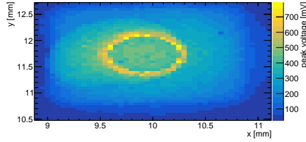
(a) \Phi_{eq} = 0 \text{ cm}^{-2} , 1700 V
