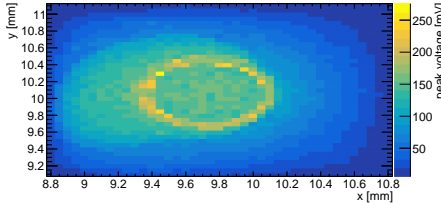
(b) \Phi_{eq} = 3 \cdot 10^{13} \text{ cm}^{-2} , 1679 V
