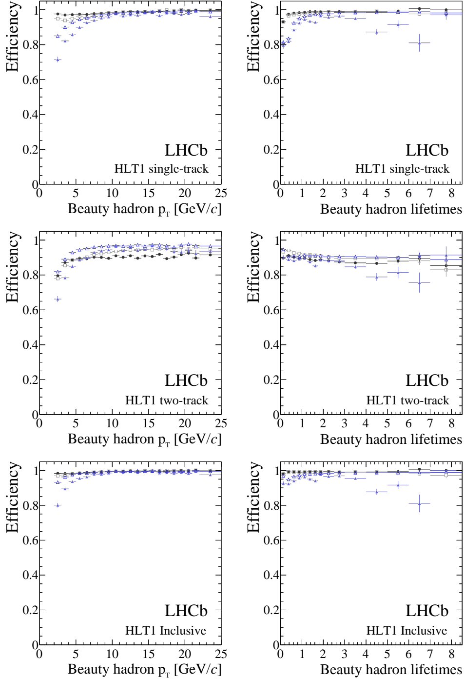
Figure 25: Efficiency of the HLT1 inclusive trigger lines as a function of (left) b -hadron p_T and (right) decay time. The decay time plots are drawn such that the x-axis is binned in units of the lifetime for each hadron in its rest frame. The plots in each column show, from top to bottom, the single-track, two-track, and combined HLT1 inclusive performance.
