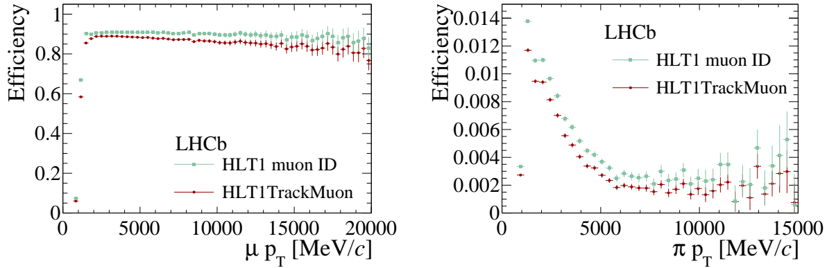
Figure 7: HLT1 muon identification efficiency for (left) muons from J/\psi \rightarrow \mu^+ \mu^- decays and (right) pions from D^0 \rightarrow K^- \pi^+ decays. Green circles show only the identification efficiency (HLT1 Muon ID) while red squares show the efficiency of the additional trigger line (named HLT1TrackMuon) requirements (see text).
