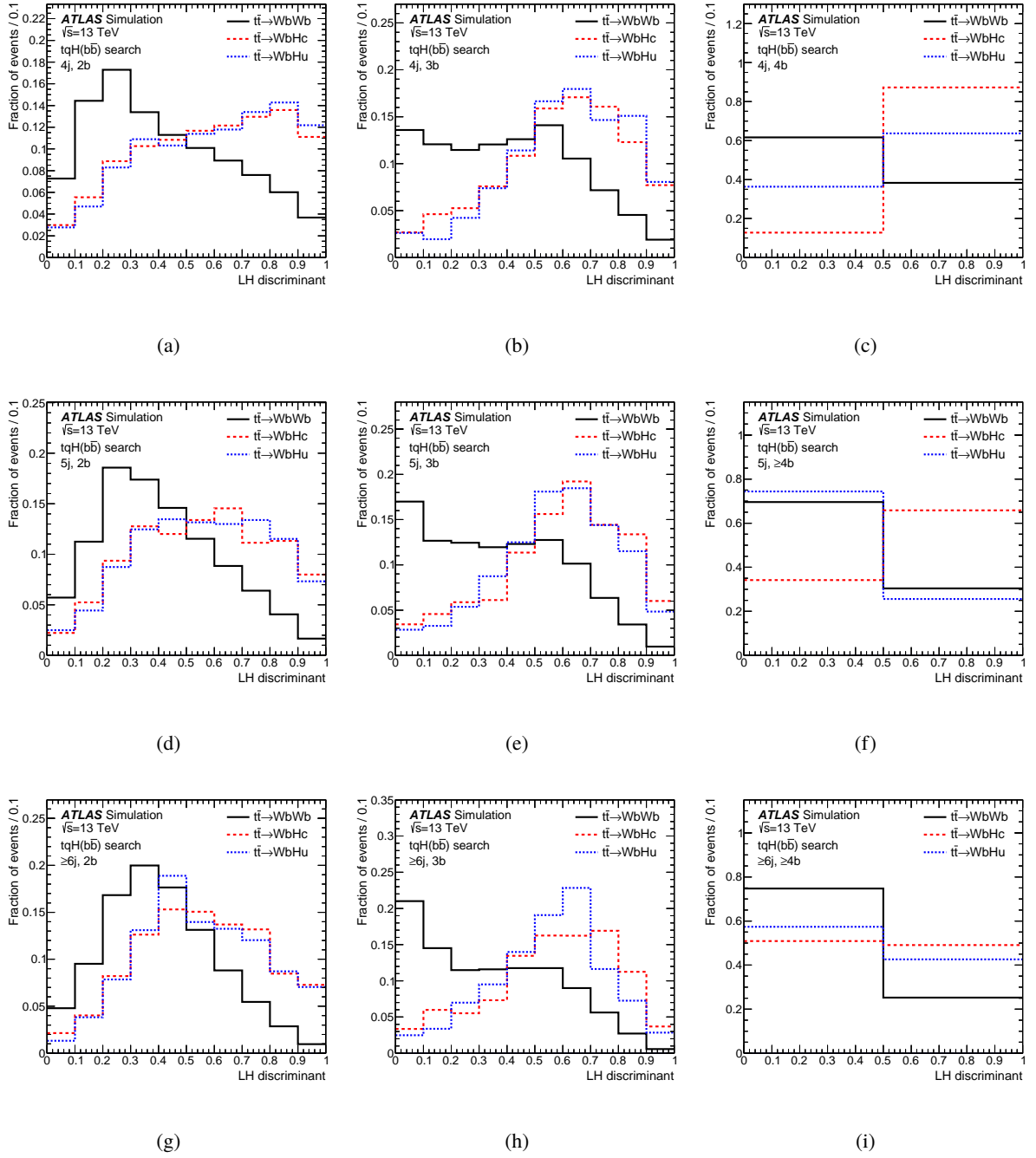
Figure 3: t\bar{t}H(b\bar{b}) search: Comparison of the distributions of the LH discriminant after preselection of the t\bar{t} \rightarrow WbHc (red dashed) and t\bar{t} \rightarrow WbHu (blue dotted) signals, and the t\bar{t} \rightarrow WbWb background (black solid) in different regions considered in the analysis: (a) (4j, 2b), (b) (4j, 3b), (c) (4j, 4b), (d) (5j, 2b), (e) (5j, 3b), (f) (5j, \geq 4b ), (g) ( \geq 6j , 2b), (h) ( \geq 6j , 3b), and (i) ( \geq 6j , \geq 4b ). In the regions with \geq 4 b -tagged jets, the signal acceptance is small, which translates into a small number of events for the simulated samples. Therefore, only two bins are used for these distributions.
