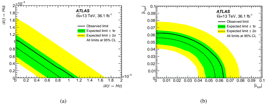
Figure 15: 95% CL upper limits (a) on the plane of \mathcal{B}(t \rightarrow Hu) versus \mathcal{B}(t \rightarrow Hc) and (b) on the plane of |\lambda_{t\mu H}| versus |\lambda_{tCH}| for the combination of the searches. The observed limits (solid lines) are compared with the expected (median) limits under the background-only hypothesis (dotted lines). The surrounding shaded bands correspond to the 68% and 95% CL intervals around the expected limits, denoted by \pm 1\sigma and \pm 2\sigma , respectively.
