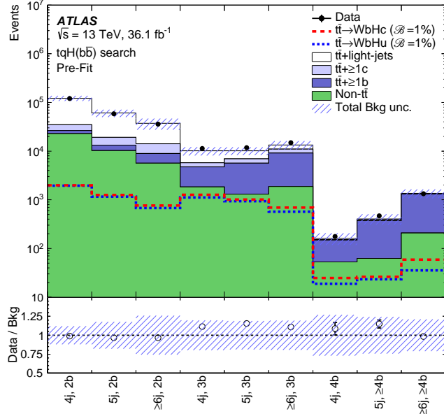
Figure 1: t\bar{q}H(b\bar{b}) search: Comparison between the data and predicted background for the event yields in each of the analysis regions considered before the fit to data (“Pre-Fit”). All events satisfy the preselection requirements, whereas those with exactly two b -tagged jets are in addition required to have a value of the likelihood discriminant above 0.6 (see Section 6.2). Backgrounds are normalised to their nominal cross sections. The small contributions from W/Z +jets, single-top-quark, diboson and multijet backgrounds are combined into a single background source referred to as “Non- t\bar{t} ”. The expected t\bar{t} \rightarrow WbHc and t\bar{t} \rightarrow WbHu signals (dashed histograms) are shown separately normalised to \mathcal{B}(t \rightarrow Hq) = 1\% . The bottom panel displays the ratio of data to the SM background (“Bkg”) prediction. The hashed area represents the total uncertainty of the background, excluding the normalisation uncertainty of the t\bar{t} + \geq 1b background, which is determined via a likelihood fit to data.
