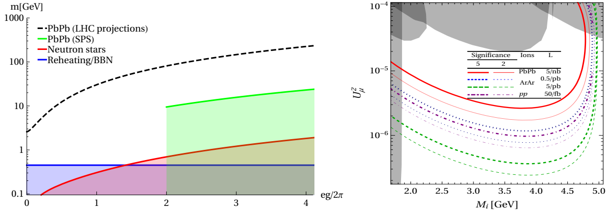
Figure 2: Left: Lower bounds for the magnetic monopole mass ( m ) vs. units of magnetic charge ( e \cdot g/2\pi ) [78]. Right: Estimated CMS reach for heavy neutrinos, with mass M_i and muon-neutrino mixing angle U_{\mu} , from B -meson decays in pp , ArAr, and PbPb collisions with equal running time [79].
