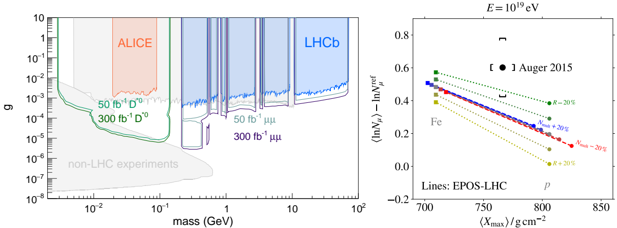
Figure 3: Left: 90% CL exclusion limits of the dark photon mixing parameter g as a function of its mass. Red and blue regions show updated projections from measurements at ALICE and LHCb [20]. Light grey bands include results from BABAR, KLOE, A1, APEX, NA48/2, E774, E141, E137, KEK, Orsay, BESIII, CHARM, HPS, NA64, NOMAD, NuCAL, and PS191 [86]. Right: Data-MC deviations in the logarithm of the number of muons produced by a 10^{19} eV CR shower versus its maximum depth in the atmosphere ( X_{\text{max}} ): Data from Auger [87] are compared to MC predictions for proton and Fe-ions CR primaries with varying values of the default MC hadron multiplicity N_{\text{mult}} and the energy fraction \alpha that goes into neutral pions. (Figure taken from [88]).
