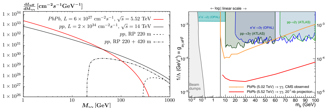
Figure 1: Left: Effective \gamma\gamma luminosity vs. photon-fusion mass in ultraperipheral PbPb and pp collisions at the LHC. In the pp case, the actually “usable” \gamma\gamma luminosity is also shown with proton tagging at 220 m (currently installed) and 420 m (proposed). Right: Exclusion limits (95% confidence level) in the ALP- \gamma coupling ( g_{a\gamma} ) vs. ALP mass ( m_a ) plane [25, 26] currently set in pp and e^+e^- (shaded areas) compared to those from PbPb UPC measurements (CMS result today [25, 26], orange curve; and projections for 20 \text{ nb}^{-1} , bottom red curve).
