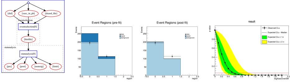
Figure 8. Example of an ATLAS recast analysis running the event selection and statistical analysis steps. This example workflow uses official ATLAS Software Group containerised environments. We see the example prefit, postfit and limit plot. The example can be found at [10].
