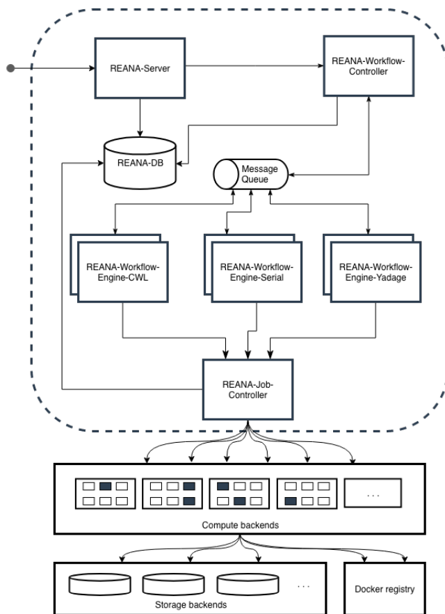
Figure 6. REANA cluster architecture and its components. The message passed to the cluster is received by API server. The diagram shows the interplay between REANA internal components and the role of the central database and message queue systems. The REANA cluster dispatches jobs on containerised clouds. Note the support for several workflow systems (CWL, Serial, Yadage). The workflow jobs use shared storage and pull necessary environment images from Docker registries.
