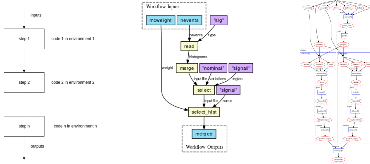
Figure 2. Examples of a serial workflow (left) and more complex Directed Acyclic Graph (DAG) workflows using CWL (center) and Yadage (right) workflow specifications. The Serial workflow is using the sequence workflow pattern where each computational step can run in a different containerised environment and the outputs of previous steps are passed along as inputs to later steps. The CWL and Yadage workflows are an example of DAG computations where the steps can be run in parallel in a "map-reduce" fashion. The full computational graphs in particle physics analyses can consist of several thousands nodes.
