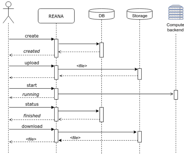
Figure 5. The sequence diagram expressing typical interaction between the REANA client and the REANA cluster.
