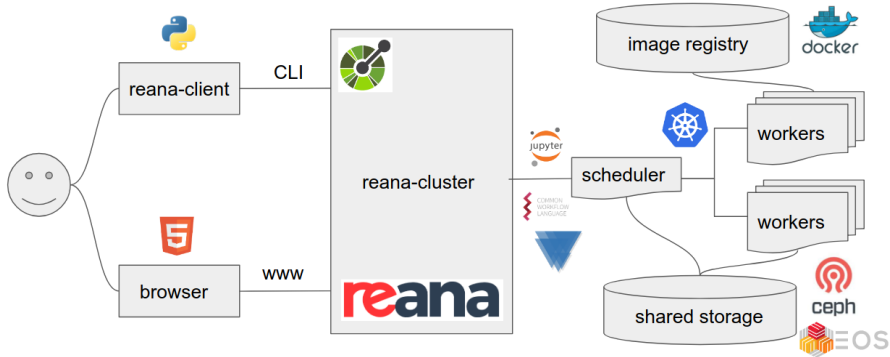
Figure 1. An overview of the REANA platform. User can interact with the platform via a command line and Web clients. The platform dispatches users’ requests to workflow engines and runs necessary tasks on the containerised cloud. The workflow tasks share the same workspace throughout the run.
