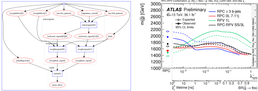
Figure 9. Left: A reinterpretation workflow for an analysis optimized for final states originating from the production of strongly interacting supersymmetric particles[12]. For reinterpretation, two separate Monte Carlo samples corresponding to different run-conditions of the LHC are processed and combined to yield an overall p-value signifying the viability of the signal in light of the observed data. Right: An earlier iteration of the same analyses was used to produce published reinterpretations[13].
