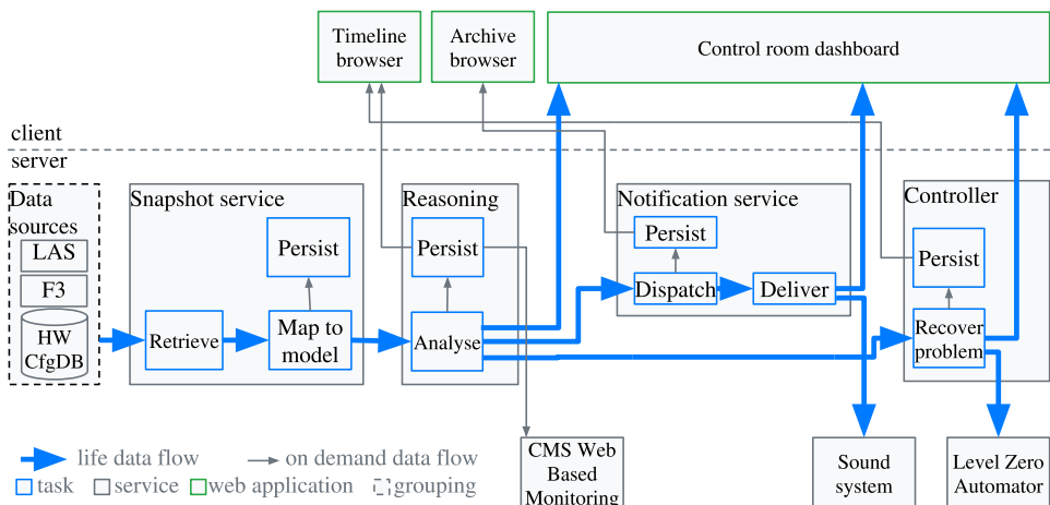
Fig. 1. Main components of the new DAQ-Expert tool. LAS: Live Access Server of the XMAS monitoring system. F3: elastic-search based monitoring of the File-based Filter Farm. HWCfgDB: CMS DAQ Hardware and Configuration Database. The server side consists of four micro-services: Snapshot Service, Reasoning Service, Notification Service, Controller.
