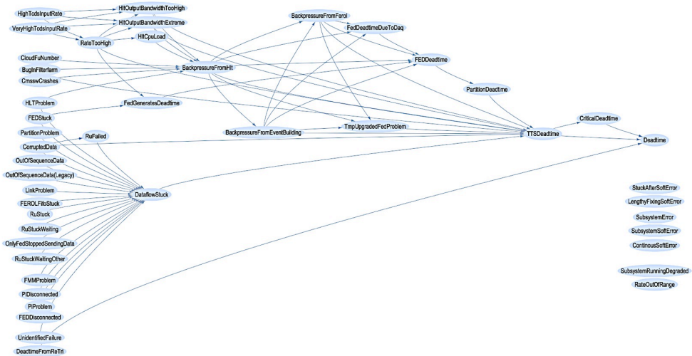
Fig. 3. Causality graph of the Logic Modules. Conditions on the right hand side may be the symptom of conditions on the left hand side.
