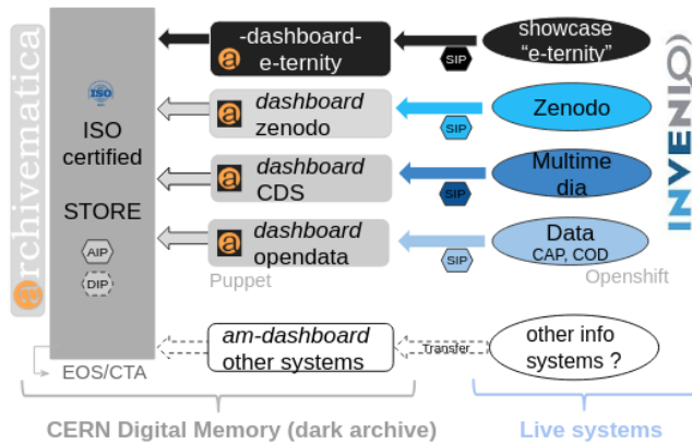
Figure 5. OAIS compliant Information Systems Architecture at CERN
