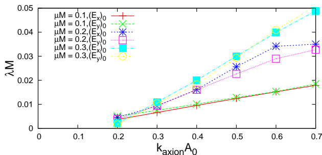
FIG. 2. The relation between the growth rate M\lambda and coupling k_{\text{axion}}A_0 , in a Minkowski background with a scalar frozen to be given by (15). The rate is extracted from the x - or y -component of the electric field at r = 60M . The instability is only present for large enough couplings, strongly suggesting the existence of a critical coupling k_{\text{axion}}A_0 . Such conclusions are substantiated by an analytical description of this system [27].
