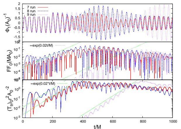
FIG. 3. Time evolution of \Phi_1 (upper panel), FF_0 (middle panel) at r = 20M and the energy flux (bottom panel) for an axion with mass M\mu = 0.2 around a BH with a = 0.5M . The coupling constant is super-critical with k_{\text{axion}}A_0 = 0.3 . The initial EM profile is described by (E_0/A_0, w/M) = (10^{-3}, 5), (10^{-3}, 20), (10^{-4}, 5) for run 7, 8, 9 respectively, and r_0 = 40 . The overall behavior and growth rate of the instability at large timescales are insensitive to the initial conditions.
