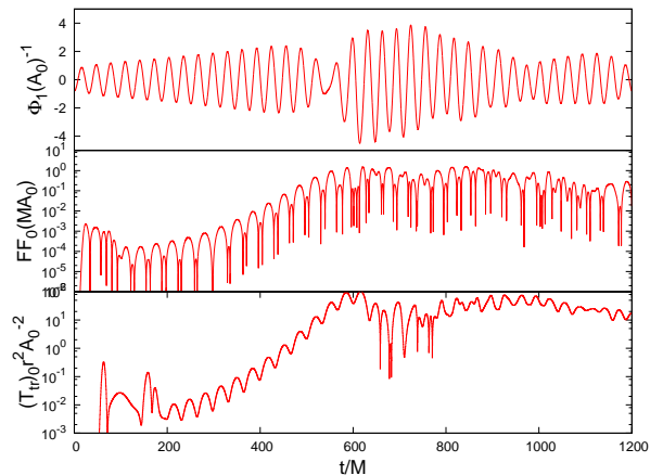
FIG. 4. Evolution of an initially sub-critical axion, driven super-critical by a superradiant-like term. After the axion becomes super-critical, an instability sets in which gives rise to a burst of EM radiation, leading to a depletion of the scalar, until a new superradiant growth set in. Our results are consistent with the triggering of periodic bursts. These results describe an axion with mass M\mu = 0.2 around a BH with a = 0.5M . The coupling constant is sub-critical k_{\text{axion}}A_0 = 0.15 . The initial EM profile is described by (E_0/A_0, w/M) = (10^{-3}, 5) and r_0 = 40 .
