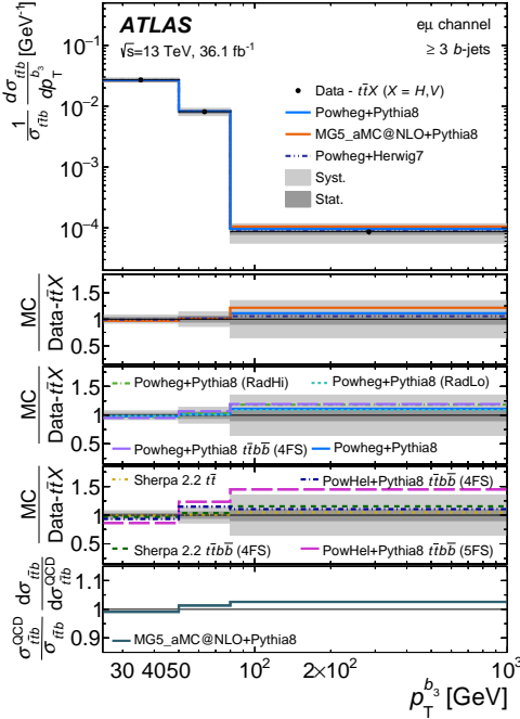
Figure 12: Relative differential cross-sections as a function of b -jets p_T for p_T -ordered b -jets in events with at least three b -jets in the e\mu channel compared with various MC generators. The t\bar{t}H and t\bar{t}V contributions are subtracted from data. (a) leading b -jet p_T , (b) sub-leading b -jet p_T , (c) third-leading b -jet p_T . Four ratio panels are shown, the first three of which show the ratios of various predictions to data. The last panel shows the ratio of predictions of normalised differential cross-sections from MADGRAPH5_aMC@NLO+PYTHIA 8 including (numerator) and not including (denominator) the contributions from t\bar{t}V and t\bar{t}H production. Uncertainty bands represent the statistical and total systematic uncertainties as described in Section 8. Events with b -jets p_T values outside the axis range are not included in the plot.
