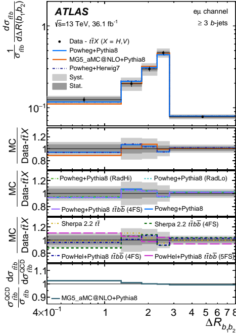
Figure 14: Relative differential cross-sections as a function of (a) m_{b_1, b_2} , (b) p_{T, b_1, b_2} , and (c) \Delta R_{b_1, b_2} of two highest- p_T b -jets in events with at least three b -jets in the e\mu channel compared with various MC generators. The t\bar{t}H and t\bar{t}V contributions are subtracted from data. Four ratio panels are shown, the first three of which show the ratios of various predictions to data. The last panel shows the ratio of predictions of normalised differential cross-sections from MADGRAPH5_aMC@NLO+PYTHIA8 including (numerator) and not including (denominator) the contributions from t\bar{t}V and t\bar{t}H production. Uncertainty bands represent the statistical and total systematic uncertainties as described in Section 8. Events with observable values outside the axis range are not included in the plot.
