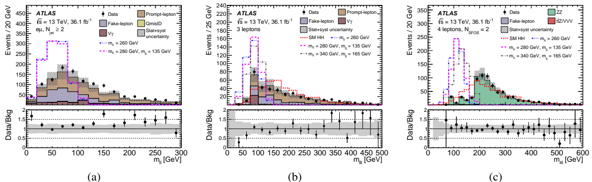
Figure 1: Distributions of the invariant mass of (a) two, (b) three, and (c) four leptons for the two, three, and four lepton channels after preselection. The charge misidentification background in the two lepton channel and the non- ZZ backgrounds in the four lepton channel are non-zero but are too small to be seen in the distributions. The shaded band in the ratio plot shows the systematic uncertainty in the background estimate. Resonant HH signal samples are denoted by m_X . The integral of each signal sample distribution is scaled to that of the expected background.
