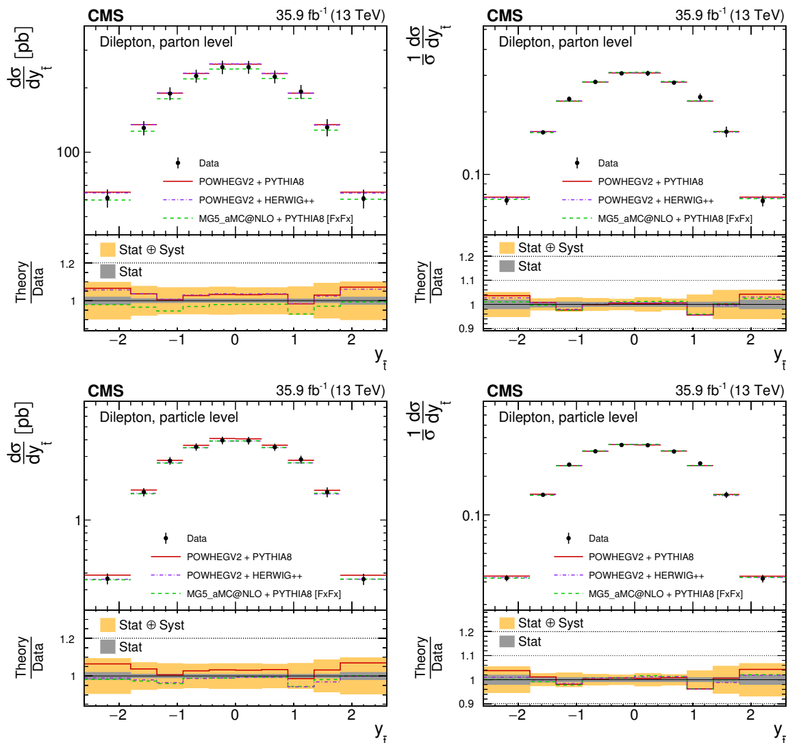
Figure 15. The differential t\bar{t} production cross sections as a function of y_{t\bar{t}} are shown for the data (points) and the MC predictions (lines). The vertical lines on the points indicate the total uncertainty in the data. The left and right columns correspond to absolute and normalised measurements, respectively. The upper row corresponds to measurements at the parton level in the full phase space and the lower row to the particle level in a fiducial phase space. The lower panel in each plot shows the ratios of the theoretical predictions to the data. The dark and light bands show the relative statistical and total uncertainties in the data, respectively.
