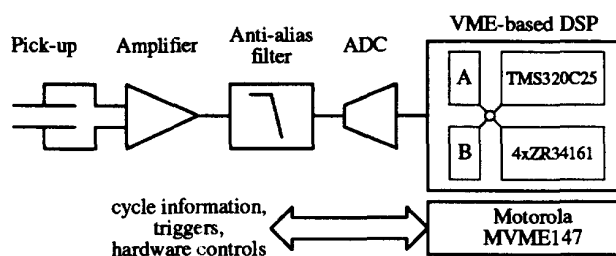
Figure 1. Hardware for the PS Q-measurement system.
