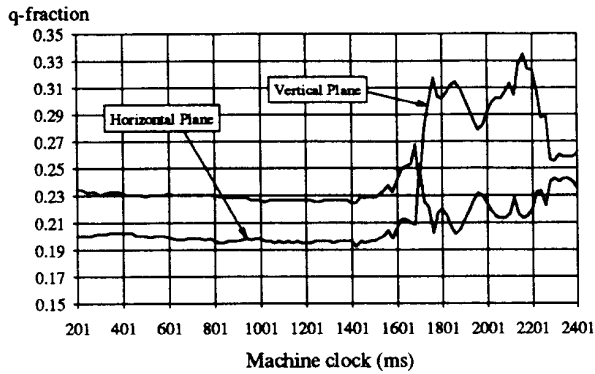
Figure 5. PS FFT Q-measurement of an LHC-type beam.
