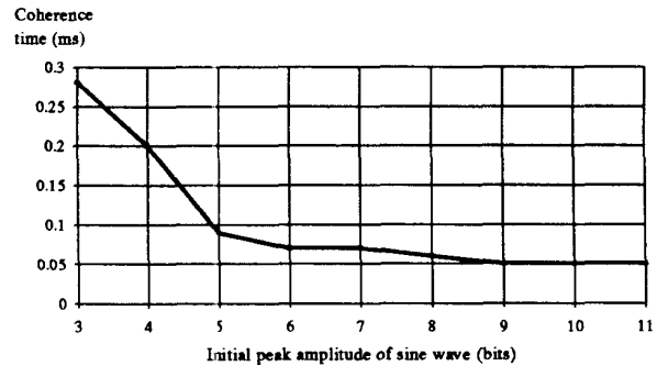
Figure 4. Maximum coherence time which a sine wave may exhibit for the q error to be less than 0.001.
