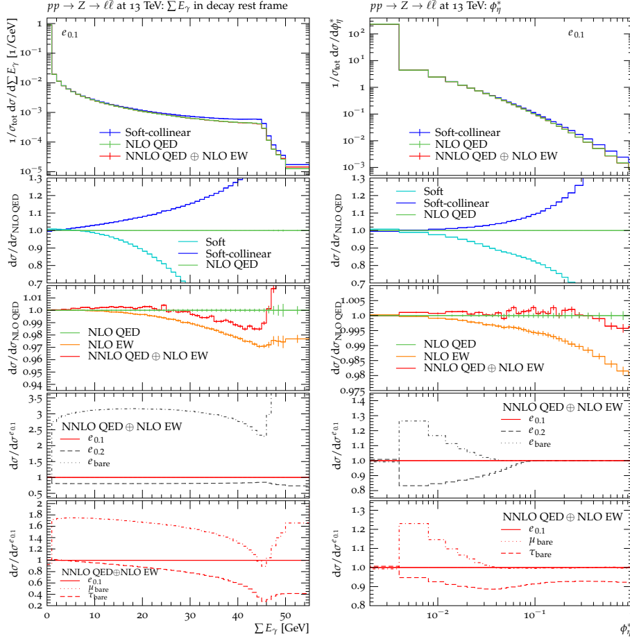
Figure 4: Plots of the sum of the photon energies in the decay rest frame, \sum_{n\gamma} E_\gamma , on the left and the \phi_\eta^* variable on the right. Predictions and labels as in Fig. 2.
