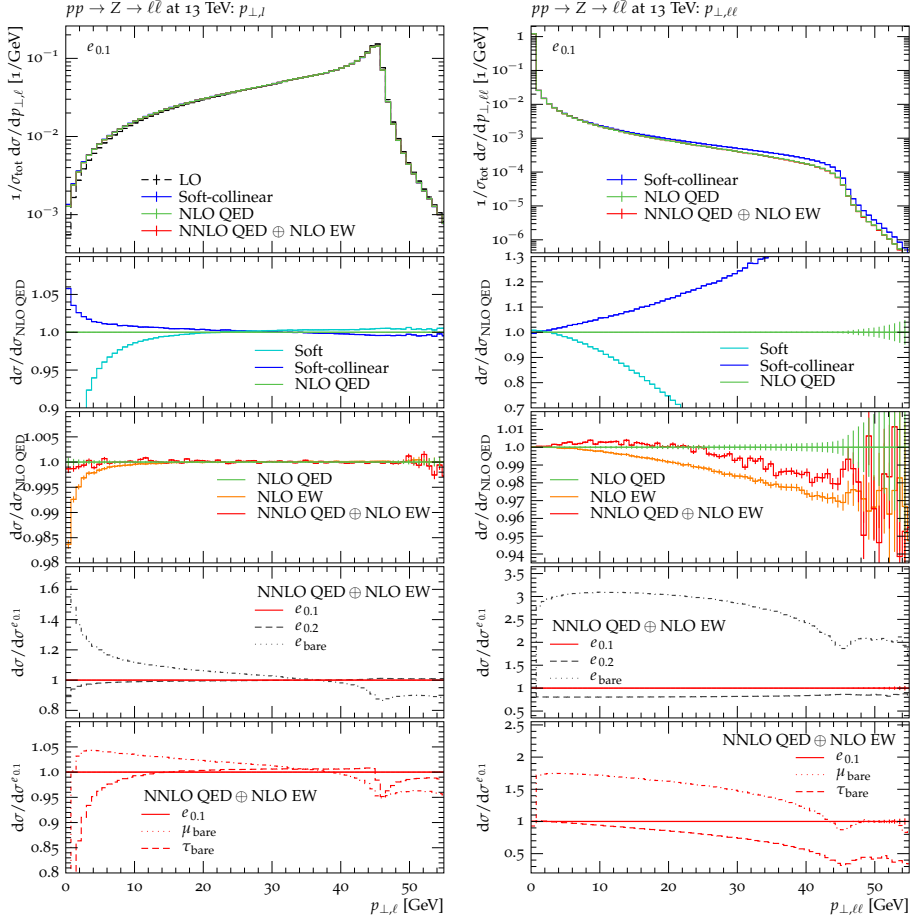
Figure 3: Plots of the transverse momentum of the leptons, p_{\perp, \ell} , on the left and the transverse momentum of the system of the two decay leptons, p_{\perp, \ell\ell} , on the right. Predictions and labels as in Fig. 2.
