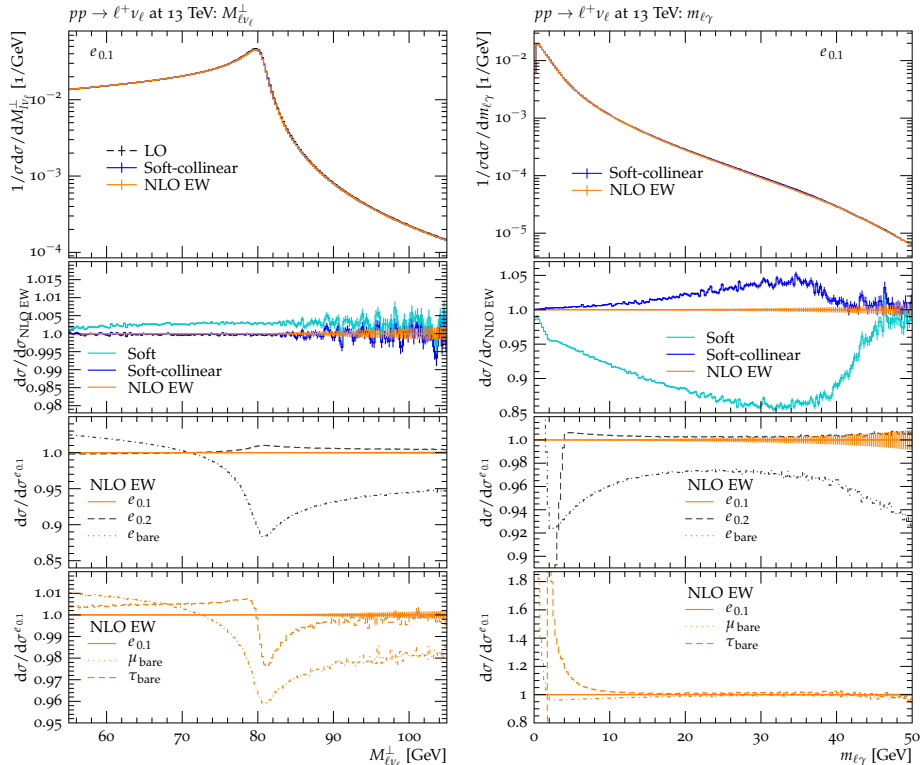
Figure 5: Transverse mass of the lepton-neutrino system M_{\ell\nu}^\perp (left) and the invariant mass of the system of the charged lepton and the nearest photon, m_{\ell\gamma} (right) in pp \rightarrow W^+ \rightarrow \ell^+ \nu_\ell . Nominal predictions are shown for pp \rightarrow W^+ \rightarrow e^+ \nu_e at LO, in soft-collinear NLO approximation and at NLO EW, where electrons are always dressed with collinear photons within \Delta R = 0.1 . The ratio plots highlight the effect of the considered higher-order corrections and the effect due to different photon dressing or lepton identity. See text for details.
