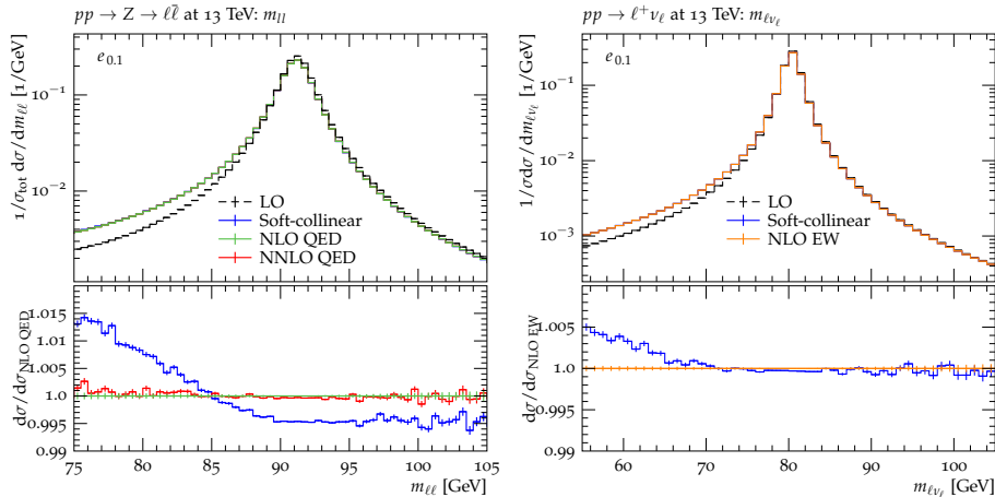
Figure 1: The invariant mass m_{\ell\ell} of the two leptons in Z -boson decays on the left and the invariant mass m_{\ell\nu} of the charged lepton and the neutrino in W -boson decays on the right are shown for the processes pp \rightarrow Z \rightarrow e^+e^- and pp \rightarrow W^+ \rightarrow e^+\nu_e respectively. Different levels of fixed order accuracy are compared. The electrons in both cases are dressed with collinear photons within \Delta R = 0.1 .
