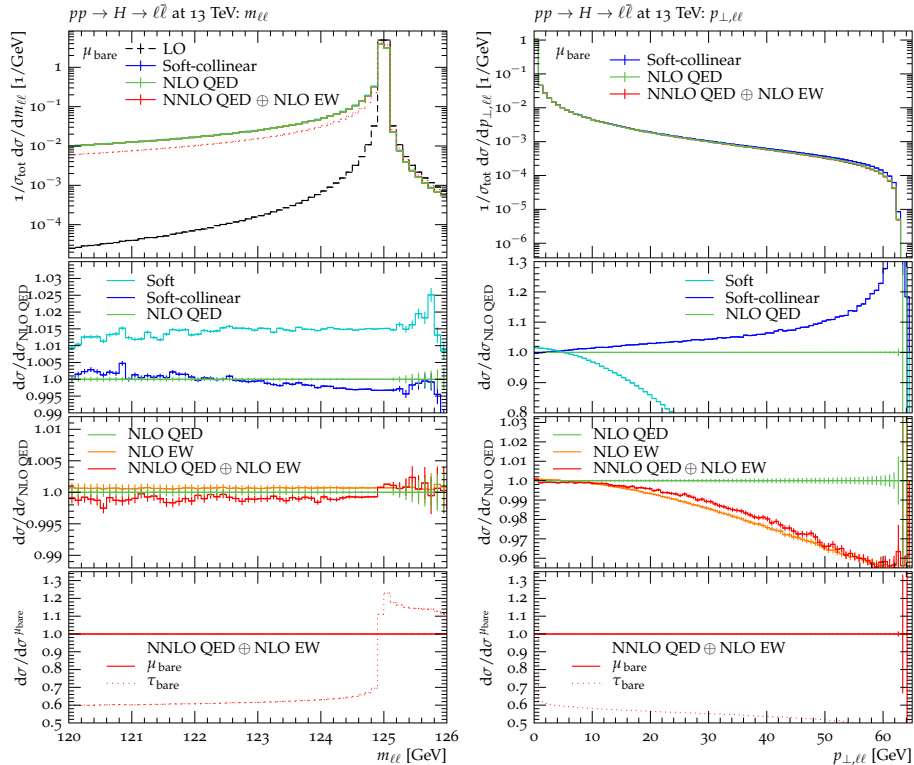
Figure 8: Plots of the invariant mass of the two decay leptons, m_{\ell\ell} , on the left and the transverse momentum of the system of the two leptons, p_{\perp,\ell\ell} , on the right in the process pp \rightarrow H \rightarrow \ell^+\ell^- . Nominal predictions are shown for pp \rightarrow H \rightarrow \mu^+\mu^- at LO, in soft-collinear NLO approximation, at NLO QED and at NNLO QED \oplus NLO EW. The ratio plots highlight the effect of the considered higher-order corrections and lepton identity. See text for details.
