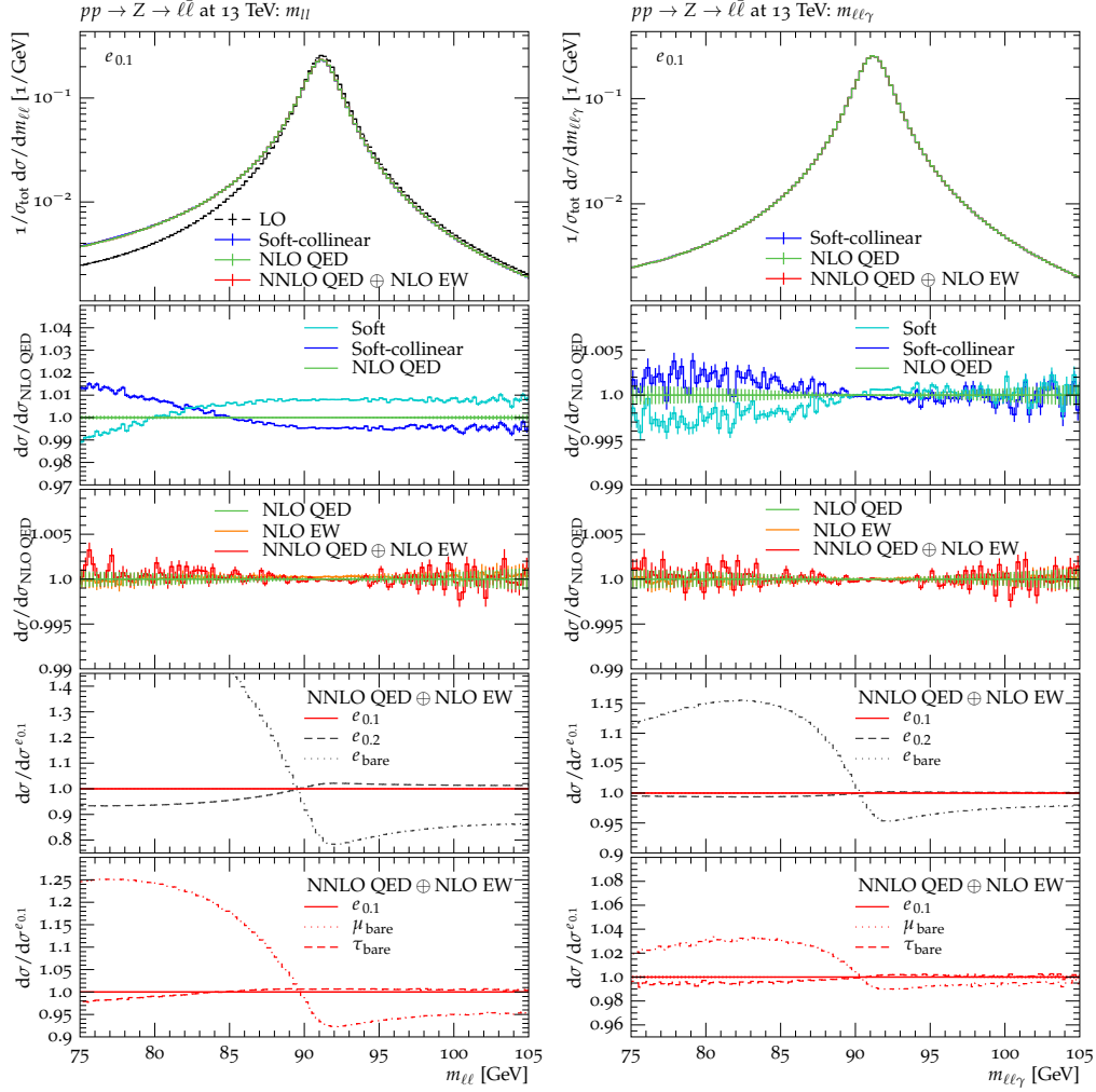
Figure 2: On the left the invariant mass of the two leptons, m_{\ell\ell} , and on the right the invariant mass of the system of the two decay leptons and the closest photon, m_{\ell\ell\gamma} , is shown for pp \rightarrow Z \rightarrow \ell^+\ell^- production. Nominal predictions are shown for pp \rightarrow Z \rightarrow e^+e^- at LO, in soft-collinear NLO approximation, at NLO QED and at NNLO QED \oplus NLO EW, where electrons are always dressed with collinear photons within \Delta R = 0.1 . The ratio plots highlight the effect of the considered higher-order corrections and the effect due to different photon dressing or lepton identity. See text for details.
