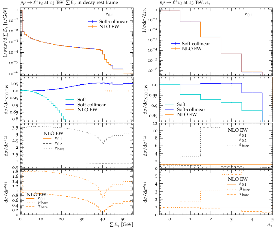
Figure 7: Plots of the sum of the photon energies in the decay rest frame, \sum_{n_\gamma} E_\gamma , on the left and the number of photons with E_\gamma > 0.1 GeV, n_\gamma , on the right. Predictions and labels as in Fig. 5.
