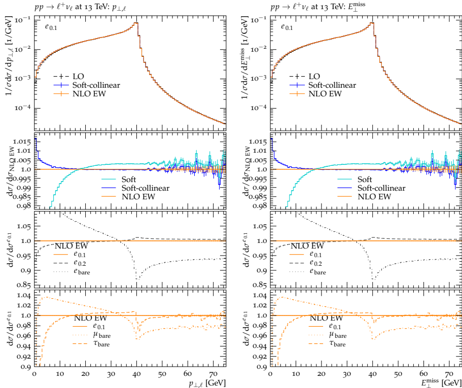
Figure 6: Plots of the transverse momentum of the charged leptons, p_{\perp,\ell} , on the left and the missing transverse E, E_{\perp}^{\text{miss}} , on the right. Predictions and labels as in Fig. 5.
