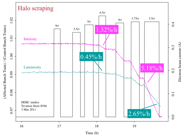
Figure 3: Normalized intensity and luminosity of the affected e-lens train with respect to the witness ones [21].
