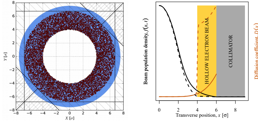
Figure 2: Concept of HEL assisted collimation: (left) the halo particles are shown by red dots, the geometrical cut performed by the horizontal–vertical–skew TCPs is represented by surrounding boxes and the hollow electron beam is depicted by the light blue ring overlapping with the halo particles and extending beyond the TCPs aperture; (right) qualitative illustration of diffusion coefficient and beam halo population with and without HEL shown by dashed and solid lines, respectively.
