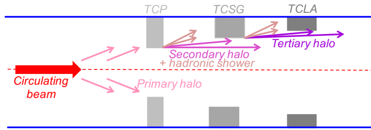
Figure 1: Working principle of the present collimation system.
