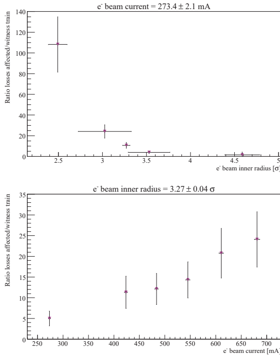
Figure 5: (top) Normalized bunch by bunch losses varying inner electron beam radius and (bottom) electron beam current.
