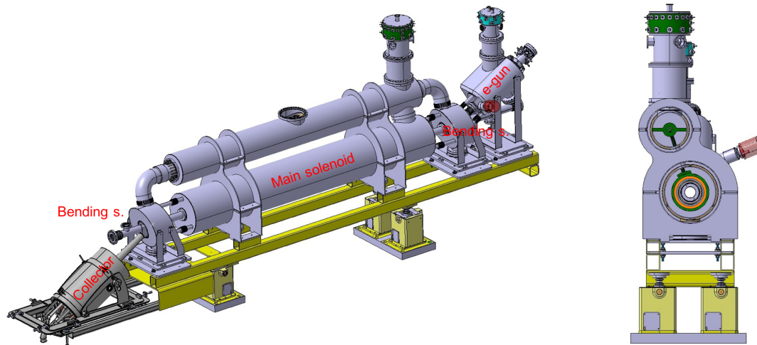
Figure 6: (left) Side and (right) front view of the present HL-LHC hollow electron lens design.
