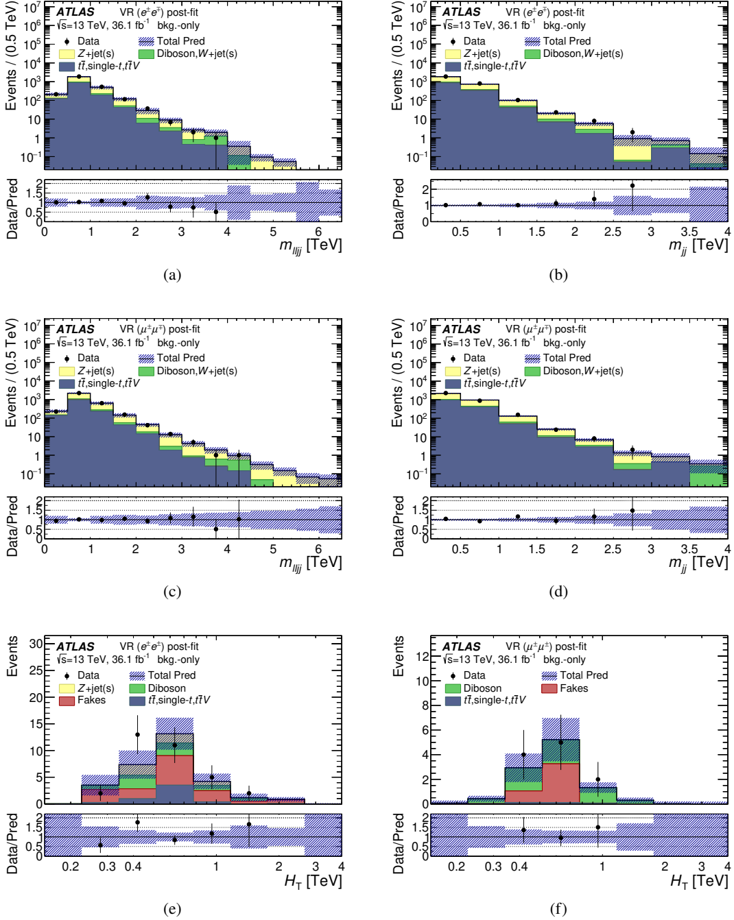
Figure 5: Distributions for data and background predictions for discriminant variables in various validation regions and channels after the background-only fit: (a) m_{lljj} in VR( e^\pm e^\mp ), (b) m_{jj} in VR( e^\pm e^\mp ), (c) m_{lljj} in VR( \mu^\pm \mu^\mp ), (d) m_{jj} in VR( \mu^\pm \mu^\mp ), (e) H_T in VR( e^\pm e^\pm ), and (f) H_T in VR( \mu^\pm \mu^\pm ). The hatched bands include all post-fit systematic uncertainties. The correlation between sources of systematic uncertainties are taken into account. The last bin in each histogram contains the overflow.
