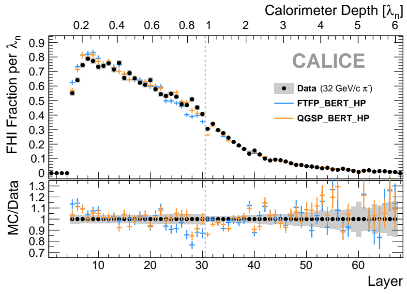
Figure 10. Distribution of the reconstructed FHI layer for 32 GeV/ c \pi^- events in data and different simulation physics lists. Energy deposits in the ScECAL are shown in layers 1 to 30, the layers 31 to 68 belong to the AHCAL.
