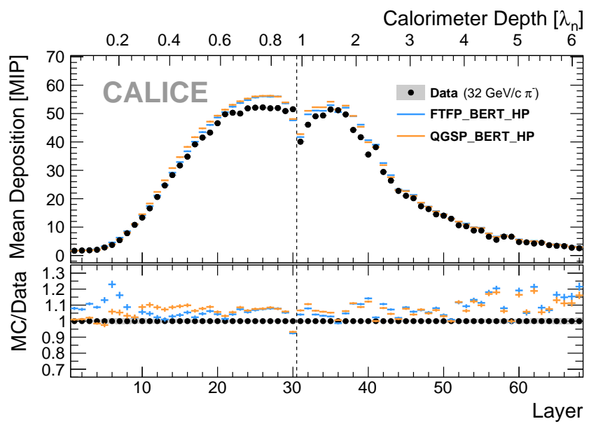
Figure 11. Average longitudinal shower profile for 32 GeV/ c \pi^- events in data and different simulation physics lists. Energy deposits in the ScECAL are shown in layers 1 to 30, the layers 31 to 68 belong to the AHCAL.
