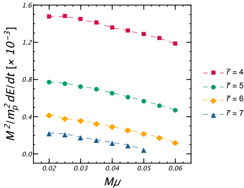
FIG. 4. GW luminosity dE/dt for the (\ell, m) = (1, 1) polar mode as a function of the 2-spin field mass M\mu for different radius \bar{r} = r_p/M of the test particle on circular orbits around the BH.
