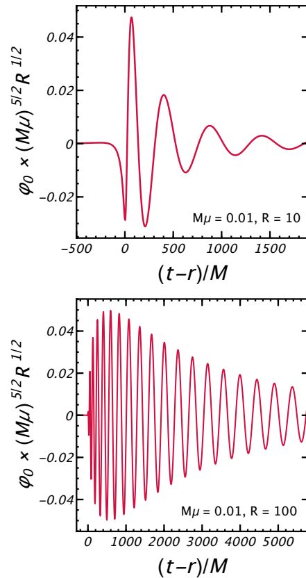
FIG. 2. Gravitational waveforms for the \ell = 0 component of the polar sector, and a radial infalling particle, as a function of the retarded time (t-r)/M . We consider M\mu = 0.01 and different extraction radius at R = (10, 100) . The waveform scales trivially with the BH mass M and the particle mass and boost m_p, \gamma , according to eq. (14).
