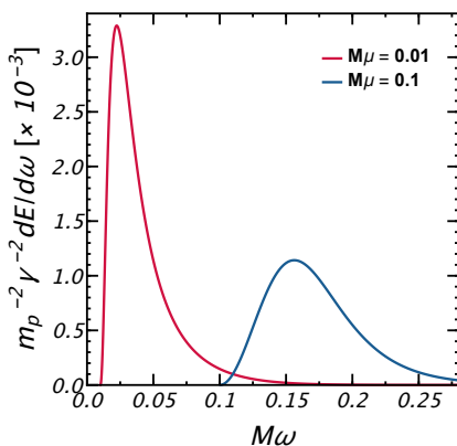
FIG. 1. GW energy spectrum dE/d\omega for the \ell = 0 polar mode, with M\mu = (0.1, 0.01) and a radial infalling particle.
