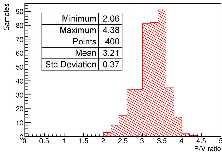
Figure 14. Distribution of the P/V ratio at room temperature for the 400 tested PMTs. Results are referred to a power supply consistent with a gain G = 10^7 .
