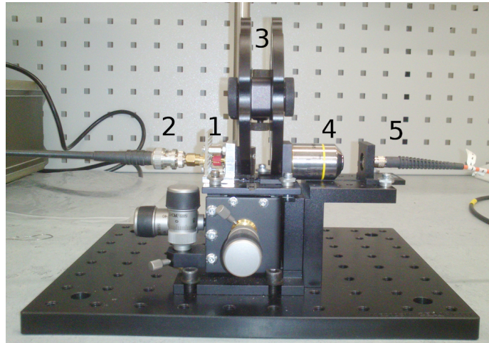
Figure 4. Picture of the adopted laser instrumentation: 1) laser diode; 2) cable from the pulser; 3) rotative supporting filters; 4) focusing lens; 5) optical fiber towards the PMT under test.
