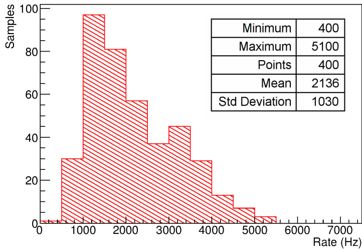
Figure 11. Dark count rate at room temperature for the 400 tested PMTs.
