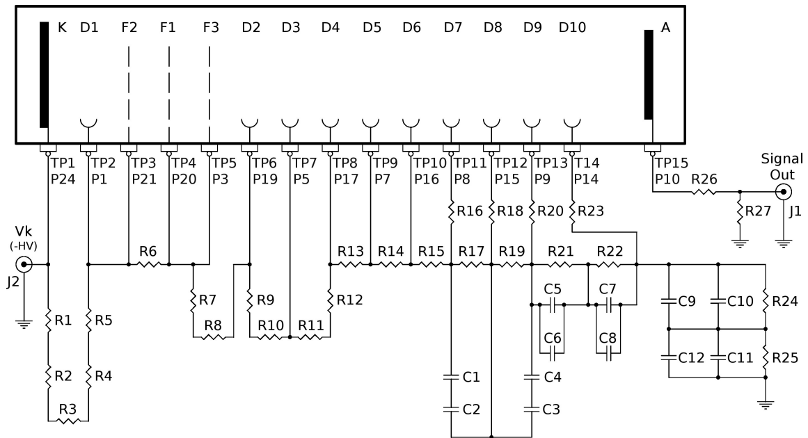
Figure 19. PMT voltage divider
