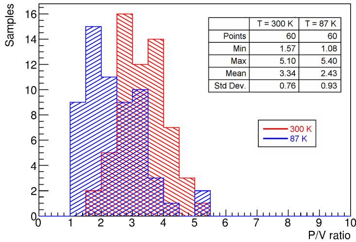
Figure 15. Comparison of the distribution of the P/V ratio at room (300 K) and at cryogenic (87 K) temperature for 60 tested PMTs. Results are referred to a power supply consistent with a gain G = 10^7 at both temperature.
