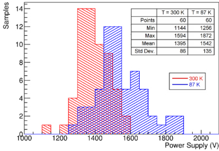
Figure 10. Distribution of voltages to attain a gain G = 10^7 both for room and cryogenic temperature
