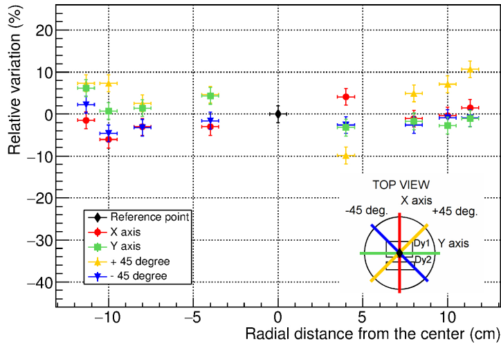
Figure 16. Variation of the photocathode response as a function of the radial distance from the window center along 4 axes oriented at 45° each other.
