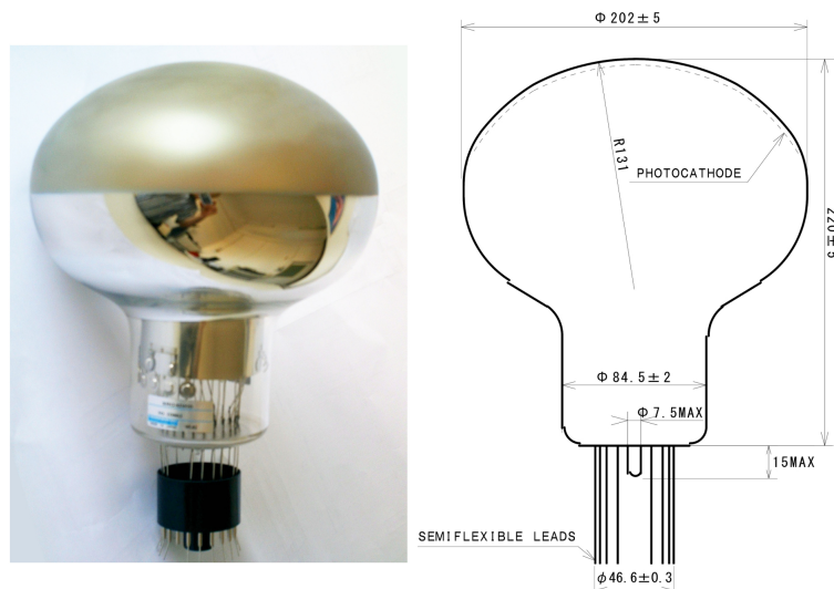
Figure 2. The PMT Hamamatsu R5912-MOD. In figure right, lengths are in millimeters
