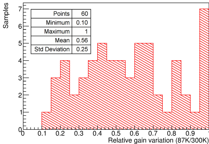
Figure 9. Relative gain variation between room and cryogenic temperature of the 60 tested PMTs. Results are referred to a power supply consistent with a gain G = 10^7 at room temperature
