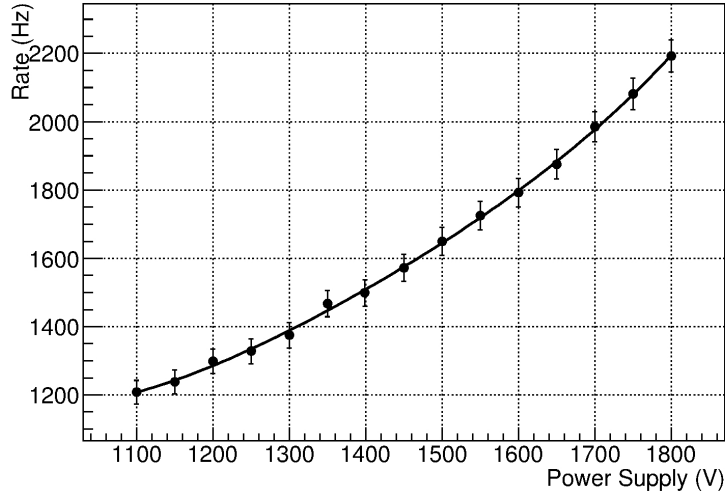
Figure 12. Example of PMT dark rate as a function of the power supply.
