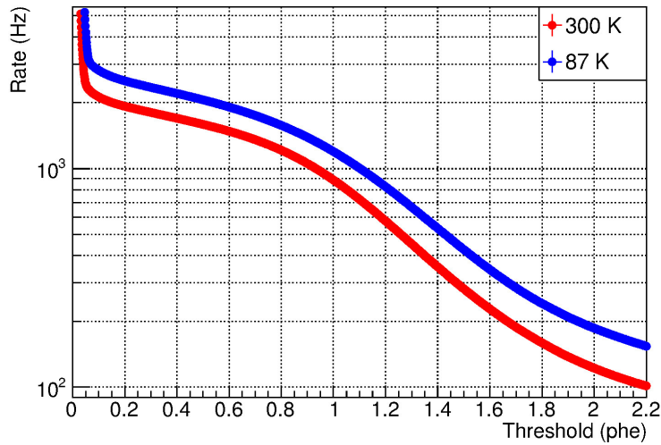
Figure 13. PMT dark count rate as a function of the discrimination threshold at room and at cryogenic temperature. The threshold value is normalized to fraction of photoelectron (phe).
