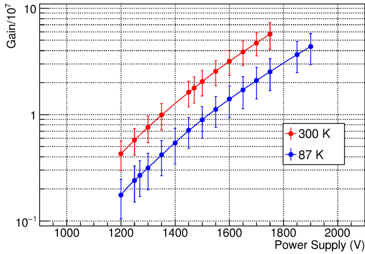
Figure 8. Example of signal amplitude (Gain) as a function of the anode voltage at room and at cryogenic temperature for a single PMT. For each measurement the peak position (dots) and the SER distribution width (vertical bars) coming from the fit are shown.
