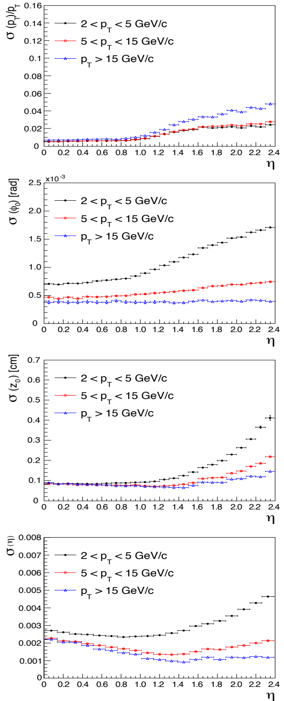
Figure 4: Track parameter resolutions for single muon events.
