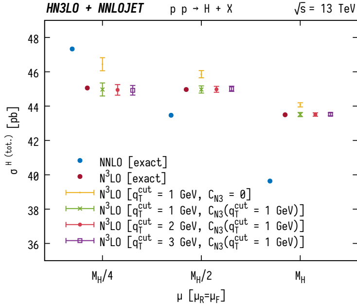
Figure 3: Total cross section of Higgs boson production, \sigma_{N^3\text{LO}}^{H(\text{tot.})} , as obtained by the q_T subtraction formalism, compared with the corresponding analytical \sigma_{N^3\text{LO}}^{H(\text{tot.})} of Ref. [13] (dark red dots). Green crosses with error bar denote the q_T subtraction prediction for q_T^{\text{cut}} = 1 GeV, red dots with error bar represents \sigma_{N^3\text{LO}}^{H(\text{tot.})} using q_T^{\text{cut}} = 2 GeV, and purple square dots with error bar having q_T^{\text{cut}} = 3 GeV. Whereas the q_T^{\text{cut}} is changed (from 1 to 3 GeV) the coefficient C_{N3} is always fixed to be the value extracted in Fig. 2 for q_T^{\text{cut}} = 1 GeV. The q_T subtraction prediction at N^3\text{LO} with the C_{N3} numerical coefficient fixed to zero (using q_T^{\text{cut}} = 1 GeV) is shown using yellow dots with error bar. The NNLO analytical Higgs boson cross section ( \sigma_{N^3\text{LO}}^{H(\text{tot.})} ) is represented by blue dots. All the cross sections are shown for three different scales: \mu \equiv \mu_R = \mu_F = \{1/4, 1/2, 1\}M_H and horizontally displaced for better visibility. The uncertainty bars in the q_T subtraction predictions are calculated with the customary propagation of statistical uncertainties.
