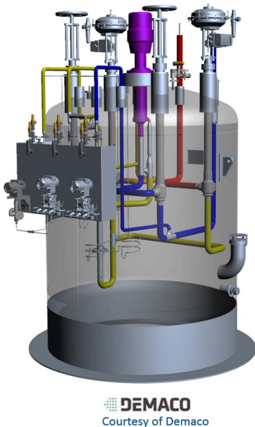
Figure 2. LAr pump.
