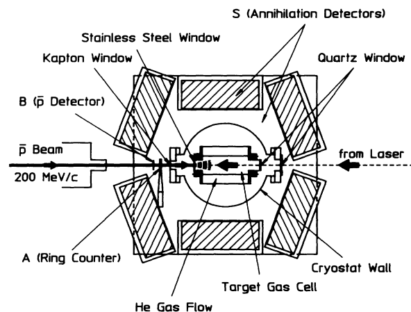
FIG. 2. Experimental setup. 200 MeV/c \bar{p} 's, passing through a beam counter ( B ) and the hole in a ring counter ( A ), are stopped in a target chamber containing helium, which is cooled to 5–10 K at 0.7–1 bar. Seven \bar{p} annihilation counters ( S , 6 sides and 1 bottom) are located around the target. Two laser beams enter the target chamber through quartz windows from the direction opposite to the \bar{p} beam.
