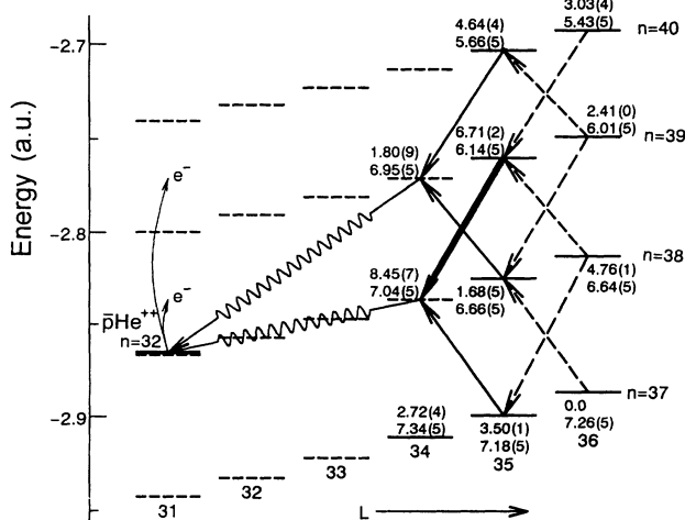
FIG. 1. Relevant energy levels versus orbital angular momentum of metastable antiprotonic helium atom \bar{p}\text{He}^+ calculated by Ohtsuki [7,8]. The levels indicated by bold lines have long lifetimes, while those indicated by broken lines are Auger dominated with short lifetimes. The calculated Auger rates (upper number) and radiative rates (lower number) per second are attached to each level, the number in parentheses being the power of 10. Possible laser-induced transitions for forced annihilation are indicated by solid arrows, with the present search candidate shown by a bold arrow. Broken arrows are used for transitions between metastable states, and \Delta l = 3 Auger (i.e., nonradiative) transitions are indicated by wavy lines.
