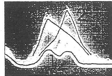
Fig. 4 Spectrum of feedforward 500 KHz/div (H) 5 dB/div (V) 1. System noise 2. Feedback off 3. Feedforward on
