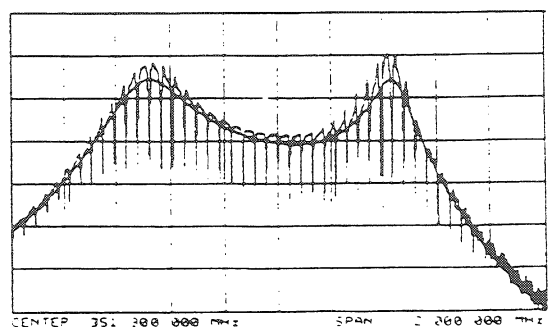
Fig. 6 Response with and without one turn feedback
