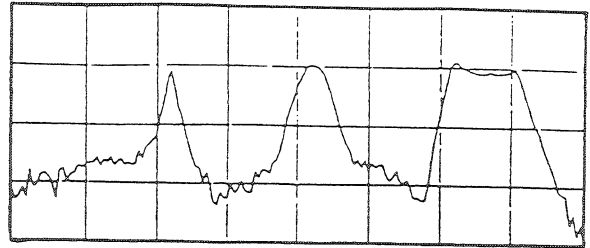
Fig. 2 4 resonances of damped cavity 349 MHz \pm 4 MHz (H); 10 dB/div (V)
