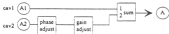
Fig. 1d Addition of 2 cavities to one turn feedback.
