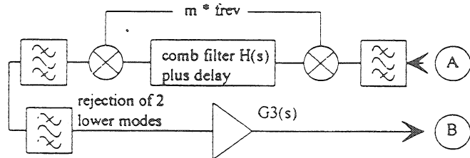
Fig. 1c Addition of one-turn feedback.
