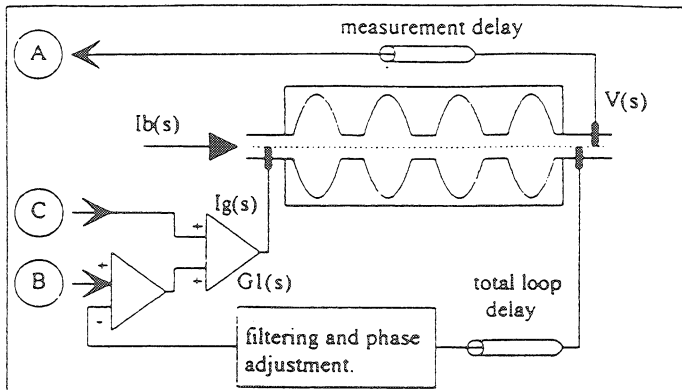
Fig. 1a RF feedback, normal operation.
