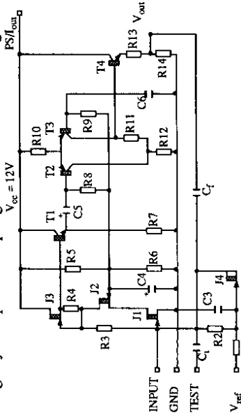
Fig. 15. Schematic of the preamplifier.
