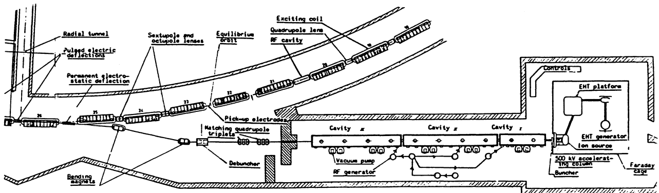
Figure 1. The Linac layout in 1960.
