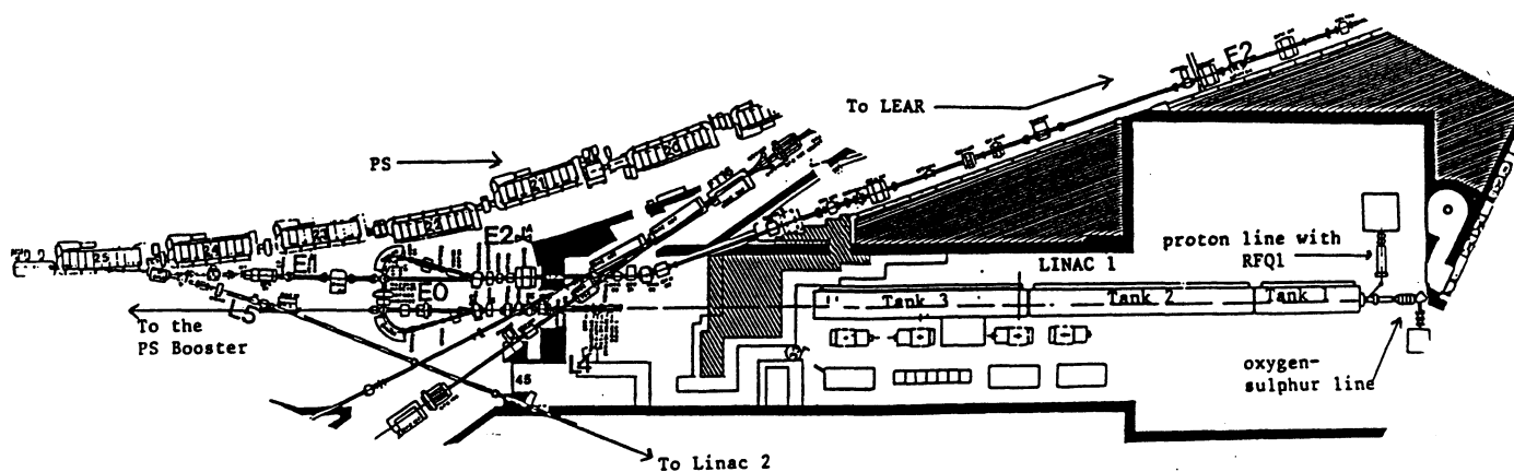
Figure 2. The Linac Layout in 1992
