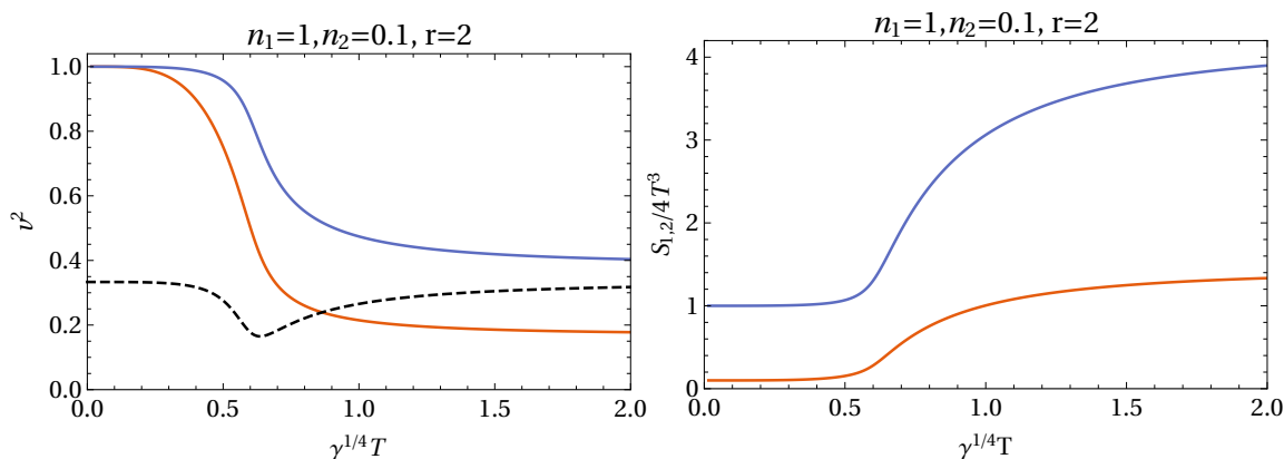
Figure 4. Unequal systems with n_1 = 1, n_2 = 0.1 and r = 2 . Left panel: light-cone velocities squared in the two subsystems ( v^2 : upper, blue line, \hat{v}^2 : lower, red line) compared to c_s^2 (dashed black line). Right panel: entropies of the two subsystems ( \mathcal{S}_1 : upper, blue line, \mathcal{S}_2 : lower, red line).
