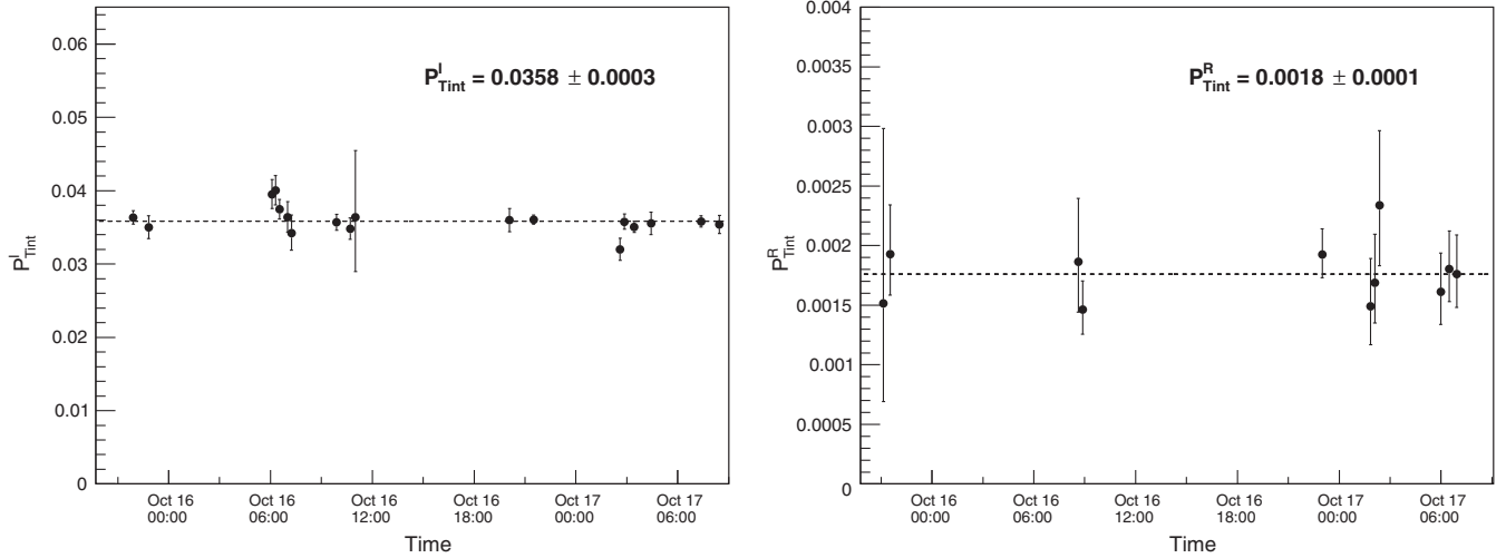
FIG. 5. Trigger interaction probabilities for the \pi^+ + C at 60 GeV/ c data set. (Left) Target inserted data set. (Right) Target removed data set.
