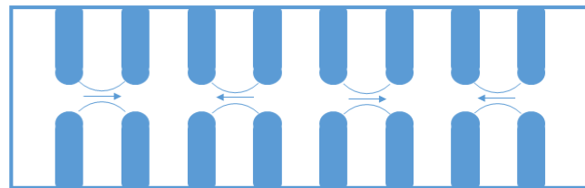
Fig. 13: Sketch of a CCL \pi/2 -mode periodic structure
