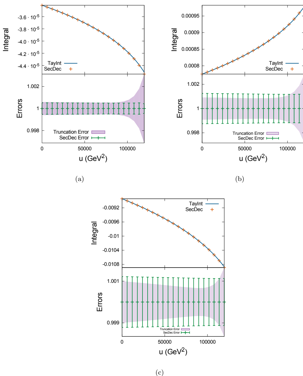
Figure 12. I_{10} below threshold, calculated with an eighth-order series expansion at; (a) \mathcal{O}(\epsilon^0) , (b) \mathcal{O}(\epsilon^1) , (c) \mathcal{O}(\epsilon^2) with m_2 = \frac{1}{\sqrt{2}}m_1 and m_1 = 173 GeV. The lower plots show the relative uncertainties of the TAYINT and numerical SECDEC results, respectively.
