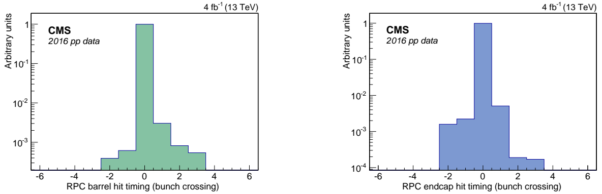
Figure 14: The bunch crossing distribution from reconstructed RPC hits in the barrel (left) and in one endcap (right), using the 2016 data.
