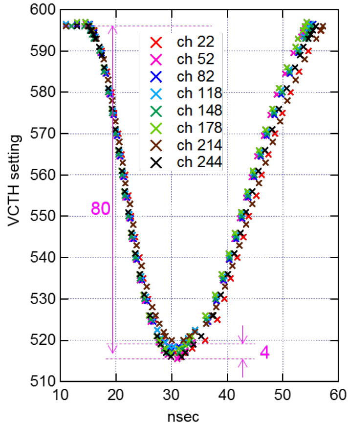
Figure 7: Pulse shapes produced by injecting a charge of 1.8 fC into the 8 externally accessible channels.
