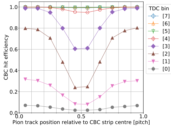
Figure 9: Hit efficiency with respect to the incident beam position relative to CBC3 strip centres, which are located at 0 and 1. Each set of data points refers to a different delay with respect to the Hit Detect signal as described in the text. The data are grouped into 3.125 ns TDC bins. Efficiency falls as events are delayed with respect to the trigger.
