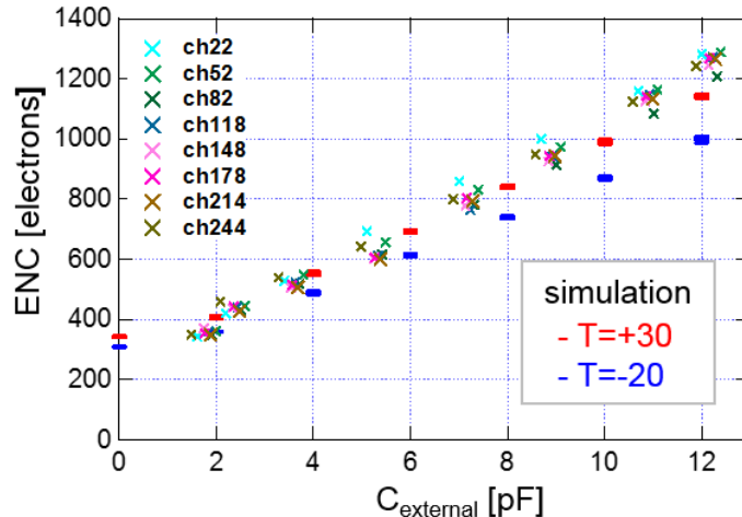
Figure 5: ENC values vs external capacitance load, compared with simulations at two temperatures.
