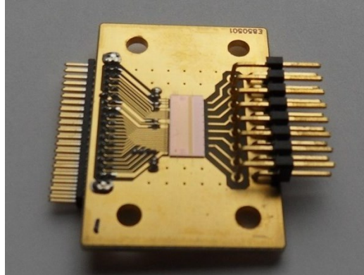
Figure 2: A CBC3 chip prepared for evaluation on a PCB using wire-bonded connections. The left-side pads are intended for probe-testing on a wafer and provide power, and control data connections. On the right-hand side, 8 signal input pads designed for bump-bonding can be connected to different load capacitances.
