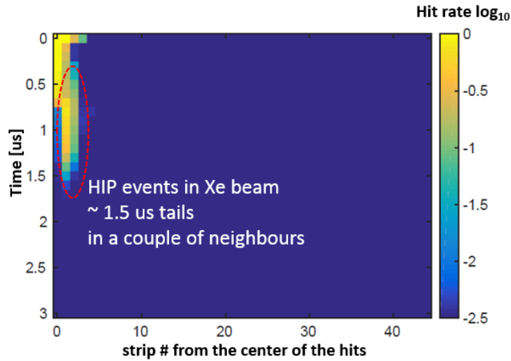
Figure 11: A 2D histogram which displays the average evolution in time of highly ionising events generated by xenon ions. The contents of the bins, normalised to the most frequently populated, is colour-coded as indicated.
