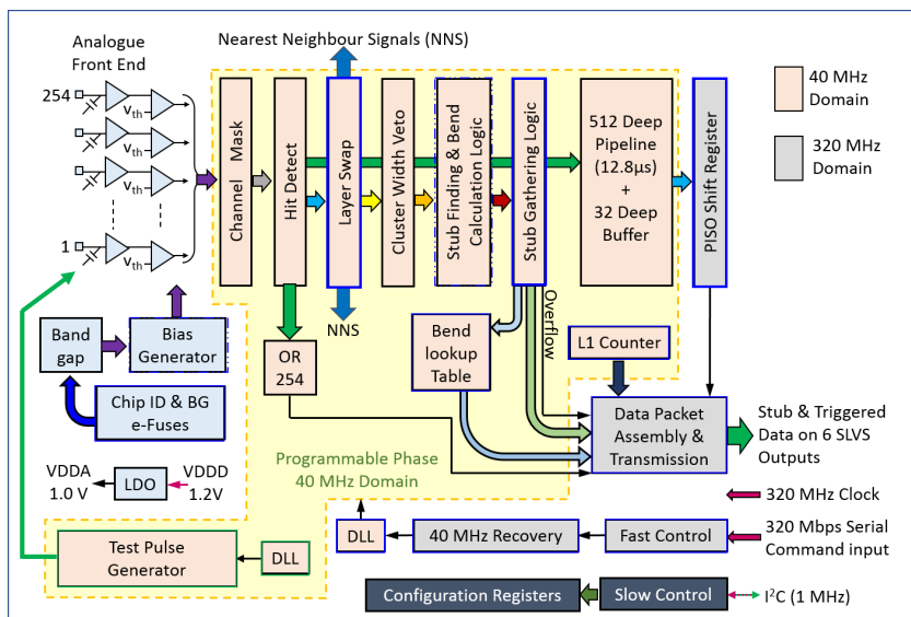
Figure 1: CBC3 architecture
