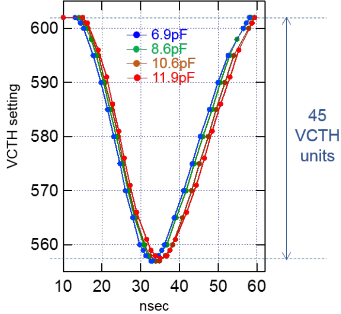
Figure 6: Pulse shapes for internal test pulse charge of \sim 1 fC with added external capacitance. 1 VCTH unit = 1.07 mV for this chip.
