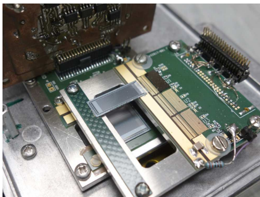
Figure 3: A CBC3 bump-bonded to a PCB, and wire-bonded to a sensor, ready for insertion in a test beam.
