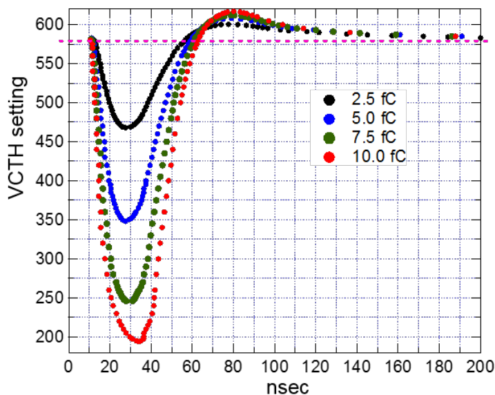
Figure 8: Pulse shapes for different values of externally injected charge. An input charge of \sim 2.5 fC corresponds to the MIP signal expected for a silicon thickness of 200 \mu\text{m} .
