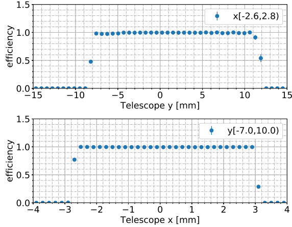
Figure 10: Hit efficiency with respect to telescope coordinate x and y , where strips are aligned parallel to y . A hit is a CBC3 cluster within 200 \mu\text{m} of the track reconstructed by the telescope. Event selection used TDC information, and events were required to be in bins 5, 6 and 7 of Figure 9.
