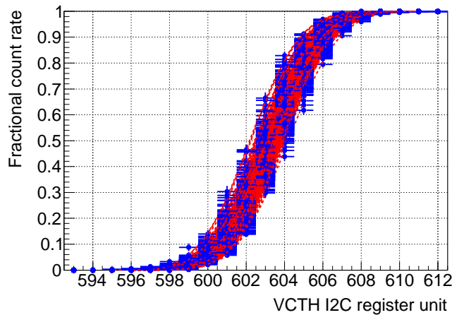
Figure 4: Pedestal s-curves for all 254 channels of one CBC3 after offset tuning. Data are the blue points, with errors and fit functions in red.
