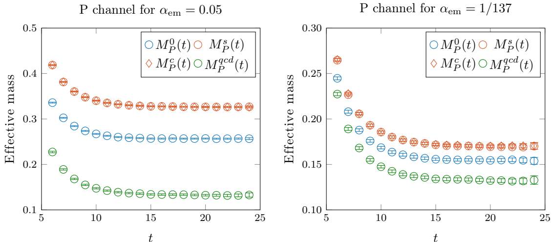
Figure 1. Effective masses for the pseudoscalar correlators at \alpha_{\text{em}} = 0.05 (left plot, blue and orange points), \alpha_{\text{em}} = 1/137 (right plot, blue and orange points), and \alpha_{\text{em}} = 0 (both plots, green points). The blue points correspond to the neutral states, M_P^0(t) . The orange points correspond to the charged states interpolated by using either the string, M_P^s(t) , or the Coulomb, M_P^c(t) , operators. The green points correspond to the states in QCD-only simulations, M_P^{qcd}(t) . The quality of the numerical signal is essentially the same for charged and neutral states, with and without QED, and it is not affected by the non-local gauge-invariant operators used in the charged channel. With these unphysical values of the bare parameters the charged-neutral mass splitting can be extracted with statistical significance even at \alpha_{\text{em}} = 1/137 .
