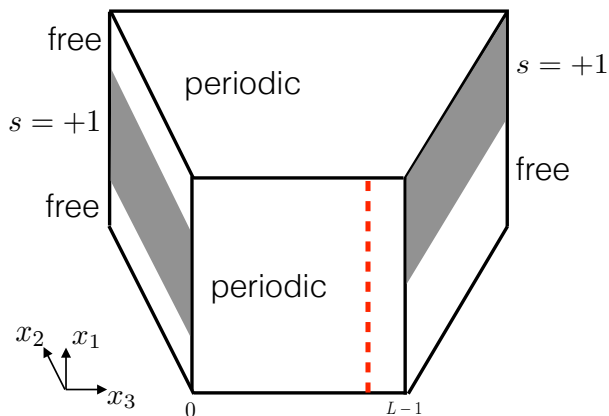
Fig. 1: The boundary conditions used in our simulation. The x_3 = 0 and x_3 = L - 1 faces have a combination of free (white) and fixed s = +1 (gray) boundary conditions. On the other faces the periodic boundary conditions are imposed. This drawing uses the Byzantine perspective only to improve visibility; the actual geometry is an L \times L \times L cube with parallel sides. The red dashed line is one possible location of the integrated observable (2.3).
