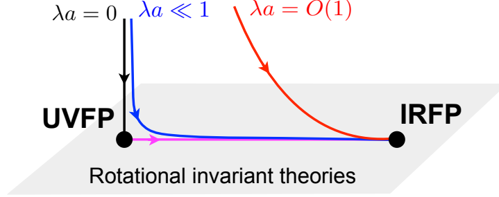
Fig. 6: Various RG flows on the critical surface of the latticized \phi^4 field theory. All flows with \lambda > 0 end up in the IRFP because we tuned the mass to its critical value. However, flows that start with \lambda a \ll 1 will first be attracted to the UVFP and from there move to the IRFP. More precisely, if the quartic coupling is parametrically small at the UV scale a , the RG flow will be controlled by the UVFP until the scale \ell_0 = 1/\lambda . At this scale, the flow transitions to the neighborhood of the IRFP. The flow with \lambda = 0 corresponds to a quadratic theory which ends in the UVFP once the rotation invariance breaking terms have decayed.
