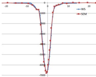
Figure 16: Grid profile (SEM) versus scanner profile (WS).
