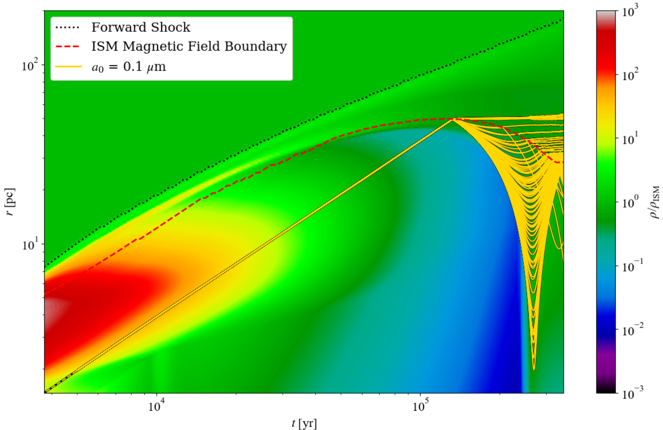
FIG. 8.— Multiple trajectories of metallic Fe-grains on a density contour. Trajectories for 100 grains (plotted in yellow) are shown with an initial grain radius of a_{\text{gr}} = 0.1\text{-}\mu\text{m} and encounter the ISM magnetic field. The grain trajectory prior to cloud crushing is shown with dashed, yellow lines and solid, yellow lines when the cloud has dissipated and the grain is exposed the SNR plasma. Note that most grains remain in the r \lesssim 50 pc region while bouncing within the shell. The FS is shown with the dotted, black curve, and the contact discontinuity between ejecta and ISM material are shown with a dashed, red line.
