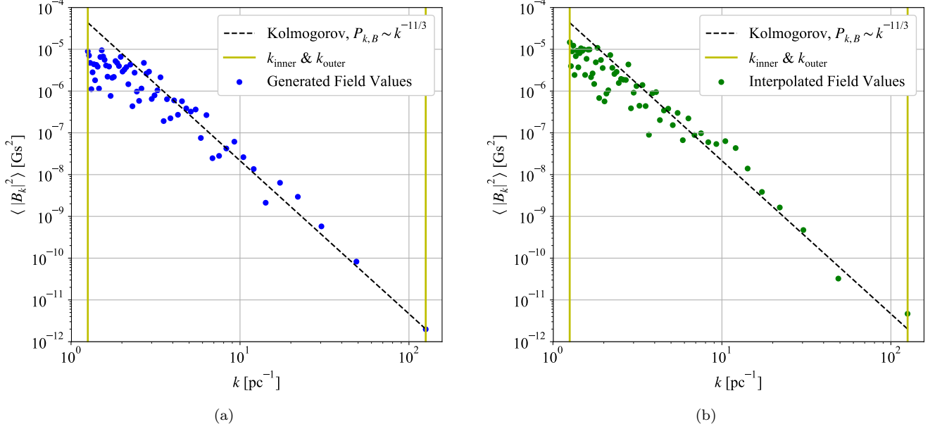
FIG. B1.— Sample power spectra for MHD turbulence. The left panel (a) shows the generated grid power spectrum for a Kolmogorov profile ( \mathcal{E}_k \sim k^{-5/3} ) with C = 1 \text{ G}^2 \text{ pc}^{17/3} , \lambda_{\text{outer}} = 5 \text{ pc} , and \lambda_{\text{inner}} = 0.05 \text{ pc} . The right panel (b) shows the interpolated field power spectrum for the same profile. The dashed line is shown for reference.
