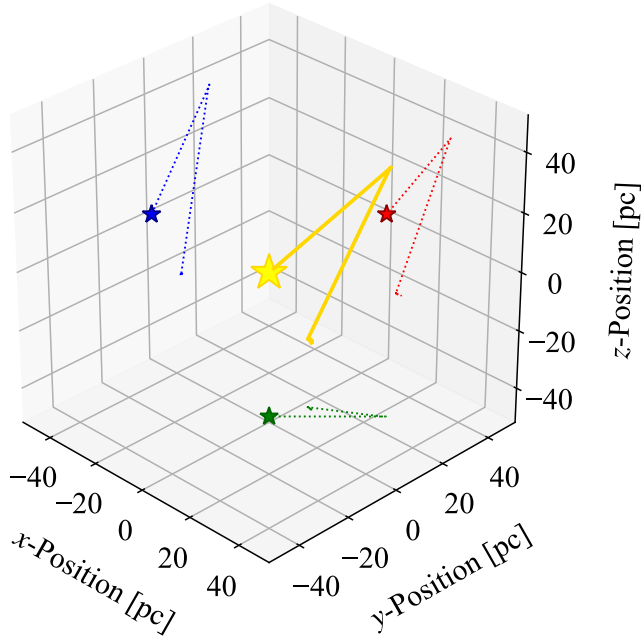
FIG. 6.— Three-dimensional plot of a sample 0.1\text{-}\mu\text{m} metallic Fe-grain. The yellow lines are the 3-D plot of the grain trajectory with the green, red, and blue lines showing the x-y , x-z , and y-z -planes respectively. The stars represent the location of the SN. Note: this is the same sample shown in Figure 5.
