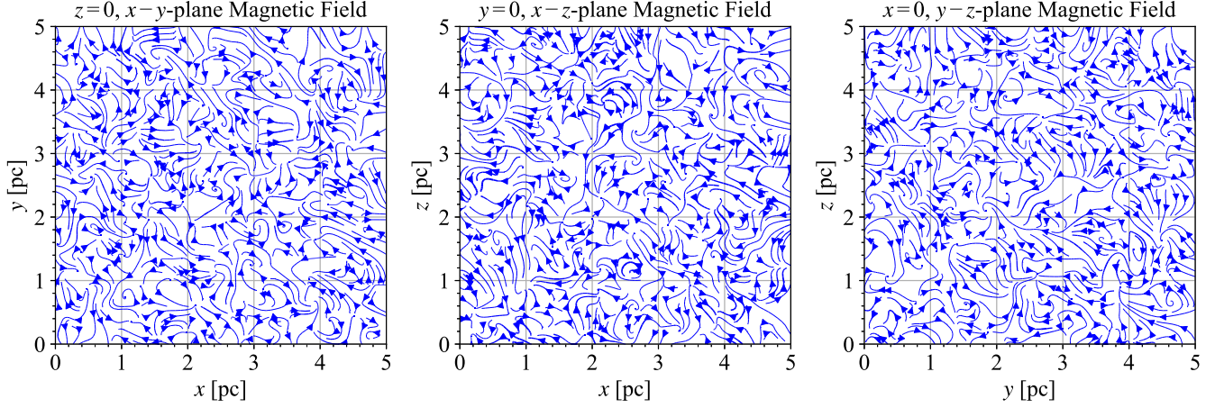
FIG. 3.— Sample turbulent field. The energy spectrum uses a Kolmogorov profile ( \mathcal{E}_k \sim k^{-5/3} ) with \mathbb{C} = 1.144 \times 10^{-13} \text{ G}^2 \text{ pc}^{17/3} , \lambda_{\text{outer}} = 5 \text{ pc} , and \lambda_{\text{inner}} = 0.05 \text{ pc} .
