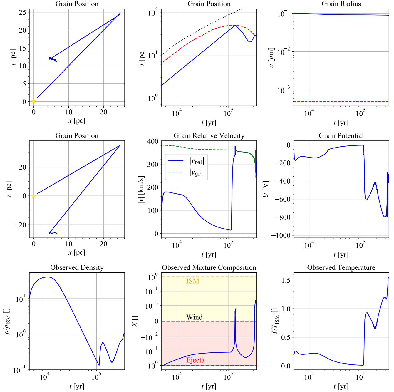
FIG. 5.— Summary of grain parameters for a sample 0.1\text{-}\mu\text{m} metallic Fe-grain. The top, left panels are projections of the grain’s positions onto the x-y - (upper left) and x-z -planes (center left) with the yellow star representing the site of the SN. The upper center plot shows the grain’s radial position with the dotted, black line indicating the position of the forward shock and the dashed, red line indicating the boundary between the pre-SN stellar wind and the ISM material and ISM magnetic field. The first reflection occurs at t \approx 1.3 \times 10^5 yr, and the grain becomes trapped in the magnetic field at t \approx 3 \times 10^5 yr. The rate of deceleration due to drag changes as the grain moves through different densities (bottom left) and is most pronounced following reflections, when the relative velocity, v_{\text{rel}} , between the grain and plasma is greatest (center). The rate of grain erosion due to sputtering remains fairly constant throughout the entire simulation (upper right), but the grain potential makes sharp fluctuations while generally staying negative (center right) and strongly mirrors the surrounding plasma temperature fluctuations (bottom right). The dashed red line on the Grain Radius plot represents the sputtering limit; below this, the grain is assumed to have been destroyed. The bottom center plot shows the pre-SN material the grain passes through; -1 is pure ejecta, 0 is pure wind, and 1 is pure ISM material with fractional values representing mixtures (there is no ISM/ejecta mixing). The grain’s reflection/trapping directly correlates to the grain’s encounters with ISM material.
