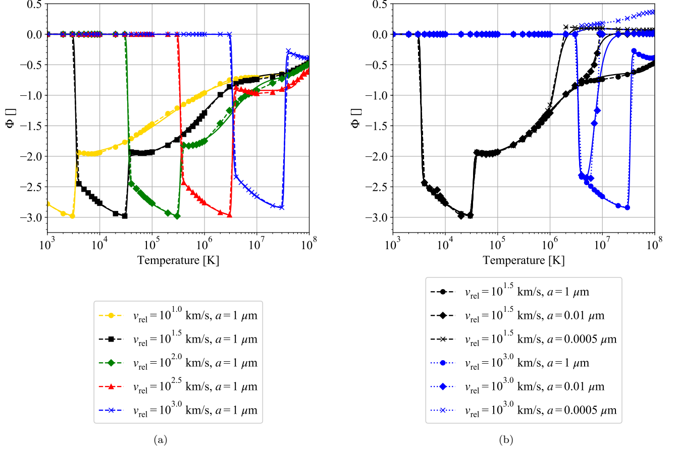
FIG. F1.— Sample potential parameters, \Phi , within the SNR for Fe grains. The left panel (a) shows the potential parameter for a 1- \mu\text{m} grain at various relative velocities, and the right panel (b) shows the potential parameter for various grain sizes. In both panels, the numerically-solved values (not including field emission) are shown with data marks and dash-dotted lines, while the analytical fit is shown with solid lines.
