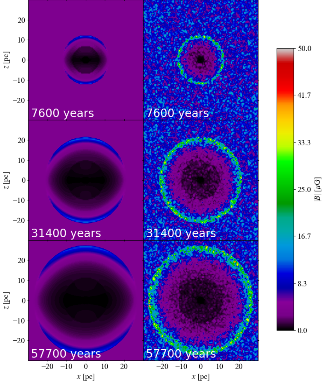
FIG. D2.— Outputs from magnetic field model for comparison to Figure 1, Balsara et al. (2001). The left column is the uniform magnetic field case; the right column is the turbulent magnetic field case. The output times are at 7600, 31,400, and 57,700 yr for the top, middle, and bottom rows, respectively.
