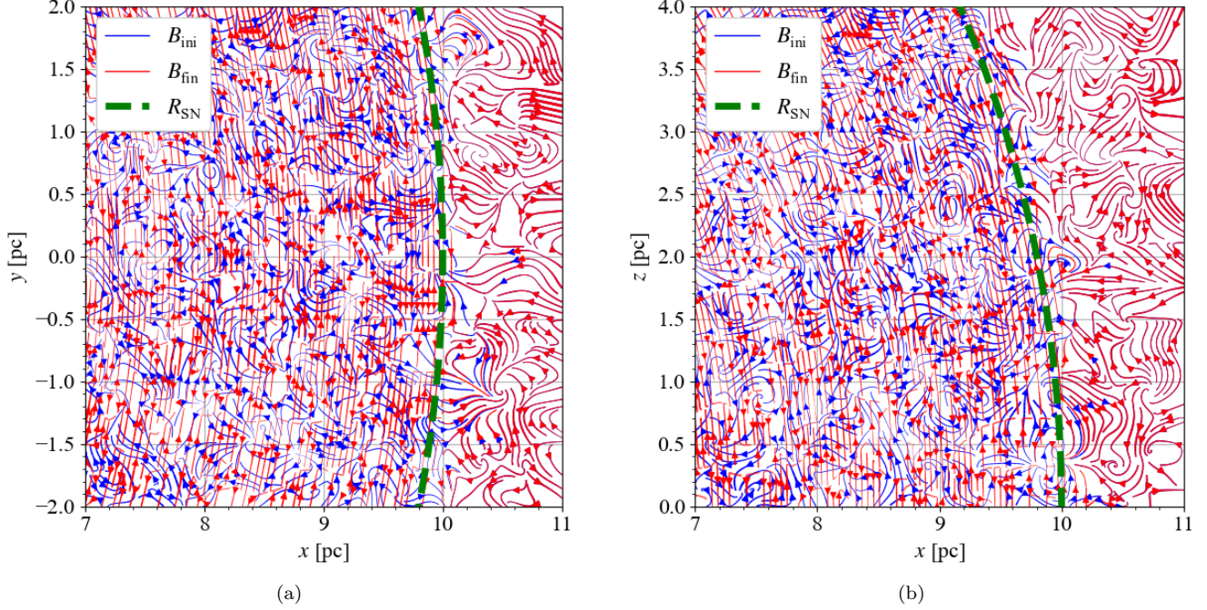
FIG. D1.— Comparison of initial and final magnetic field conditions after the passage of a shock wave with a generic Sedov profile. The initial magnetic field (shown in blue) is stretched and compressed (red lines) as the shock wave passes through the medium. Here the spherical shock is centered at the origin and has a radius of 10 pc (dashed green line). [Note: The slight variations between the initial and final magnetic fields just ahead of the shock wave are a product of the plotting algorithm not the calculation.]
