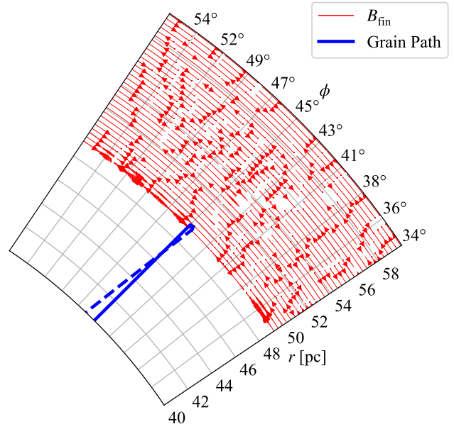
FIG. 7.— The azimuthal trajectory of a sample 0.1\text{-}\mu\text{m} metallic Fe-grain along its initial radial direction. The grain path is shown as a solid blue until reflection, and a dashed, blue line afterwards. The red lines are the magnetic field lines at the moment of reflection ( t \approx 130 kyr, r \approx 50 pc). Note the stretching of the magnetic field lines parallel to the FS and the lack of a magnetic field interior to 49 pc representing pre-SN stellar and wind material. Because of mixing of the wind and ISM material, the magnetic field gradually increases in strength, until strong enough to reflect the dust grain.
