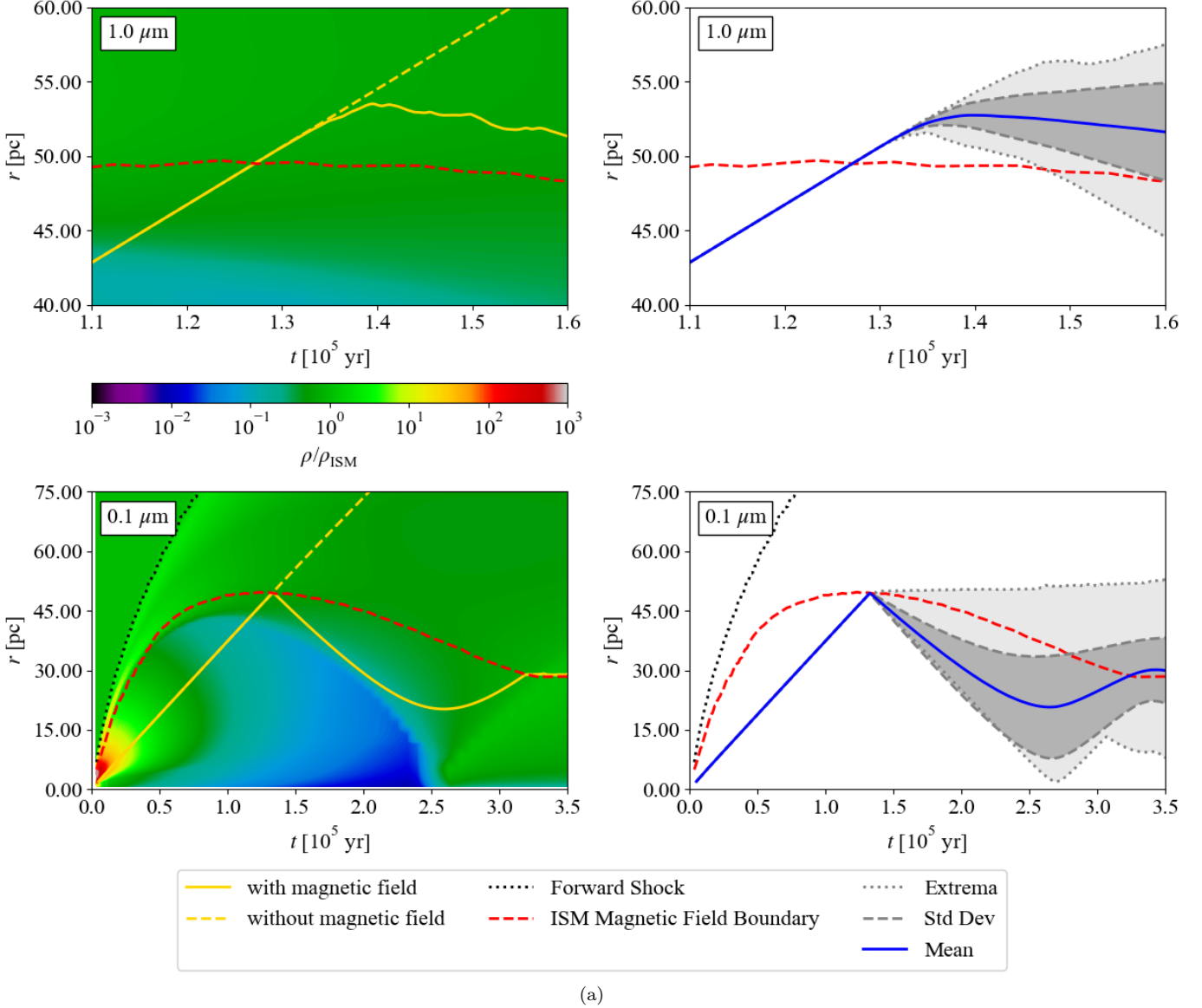
FIG. 4.— Sample trajectories of metallic Fe-grains of varying initial sizes on a density contour (left) and means/standard deviations/extrema of trajectories (right). The \gtrsim 0.05\text{-}\mu\text{m} grains showed little influence by drag, traveling on similar trajectories when no magnetic field is present, but experiencing strong interactions in the presence of a magnetized ISM. Panel (a): Most 1\text{-}\mu\text{m} grains became trapped in the ISM magnetic field; their greater mass contributing to greater penetration before capture, but preventing later escape. In contrast, the 0.1\text{-}\mu\text{m} grains experience mostly reflections at the first contact with the ISM magnetic field, while most grains become trapped at the second contact (although some grains do show additional reflections). Panel (b): The \lesssim 0.05\text{-}\mu\text{m} grains showed increasing influence by drag, delaying interaction with the magnetized ISM. Most 0.05\text{-}\mu\text{m} grains became trapped in the ISM magnetic field, although occasional reflections did occur. The 0.005\text{-}\mu\text{m} grains demonstrated no reflections and were completely trapped by the ISM magnetic field. Below \leq 0.004\text{-}\mu\text{m} , drag and sputtering on dust grains becomes significant, with the smallest grains never reaching ISM material before being completely sputtered. The standard deviation assumes a normal distribution.
