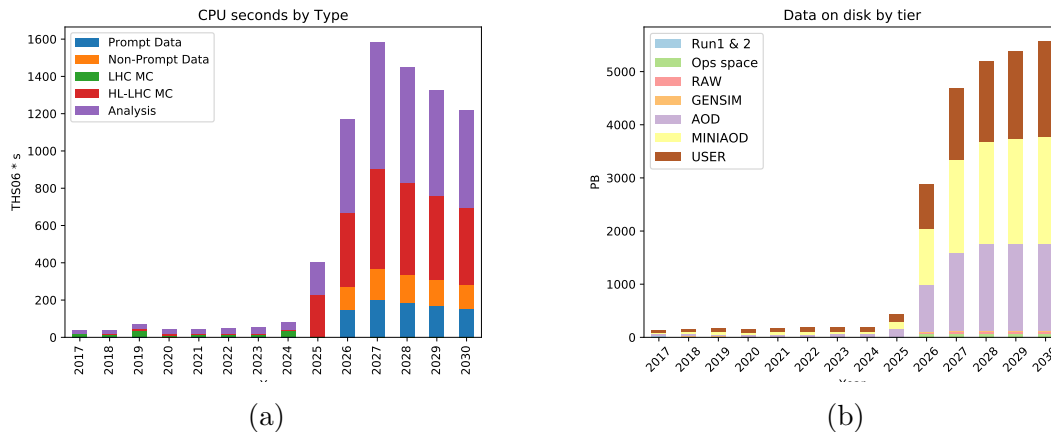
Figure 3: CMS estimated CPU (3a) and disk space (3b) resources required into the HL-LHC era, using the current computing model with parameters projected out for the next 12 years [39].
