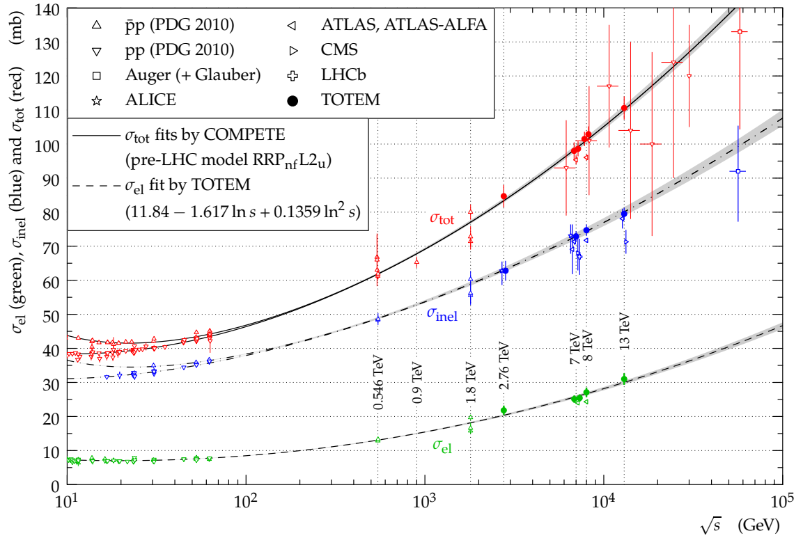
Fig. 4: (color). Overview of elastic ( \sigma_{el} ), inelastic ( \sigma_{inel} ), total ( \sigma_{tot} ) cross section for pp and p\bar{p} collisions as a function of \sqrt{s} , including TOTEM measurements over the whole energy range explored by the LHC [1, 2, 4–6, 10, 13, 22–31]. Uncertainty band on theoretical models and/or fits are as described in the legend. The continuous black lines (lower for pp , upper for p\bar{p} ) represent the best fits of the total cross section data by the COMPETE collaboration [32]. The dashed line results from a fit of the elastic scattering data. The dash-dotted lines refer to the inelastic cross section and are obtained as the difference between the continuous and dashed fits.
