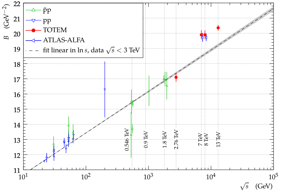
Fig. 7: (color). The nuclear slope B for pp and p\bar{p} elastic scattering as a function of \sqrt{s} . It should be understood that while B is defined at t = 0 , the experimental measurements are actually averaging the slope, hence they depend on the chosen t -range and on the deviations of the data from a pure exponential. While fluctuations beyond the experimental error bars should thus be expected, the deviation for \sqrt{s} > 3 TeV from the linear extrapolation is highly significant [1, 5, 6, 10, 22, 27, 28].
