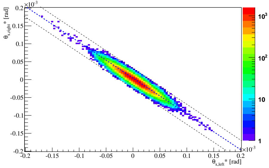
Fig. 1: (color) Analysis cut in the horizontal scattering angle \theta_x^* . The blue and black dashed lines represent the mean and the 4\sigma cuts, respectively.
