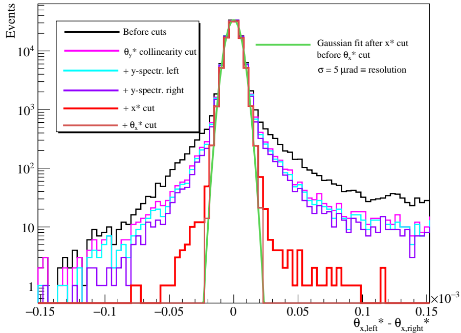
Fig. 2: (color) The distribution of the horizontal scattering angle difference reconstructed from the left and the right arm. The distribution is shown before any analysis cut (black solid line) and after each analysis cut.
