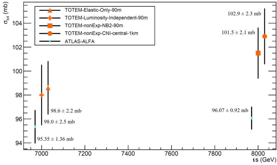
Fig. 5: (color). Focus on the 7 - 8 TeV range showing the comparison of the pairs of TOTEM measurements which represent the broadest exploration of different methods, data sets, t -range (with or without Coulomb-nuclear interference) and descriptions of the nuclear slope with the ATLAS-ALFA measurements [2, 4, 10, 13, 27, 28].
