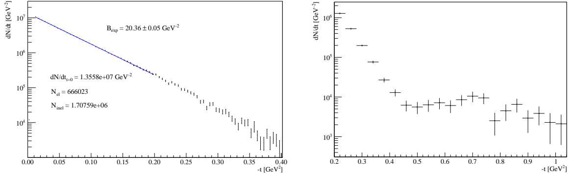
Fig. 3: Differential elastic rate dN_{\text{el}}/dt at \sqrt{s} = 13 TeV (full physics corrections included) of dataset DS2 with the exponential fit between |t|_{\text{min}} and |t|_{\text{max}} . The right panel shows the data in the dip region.
