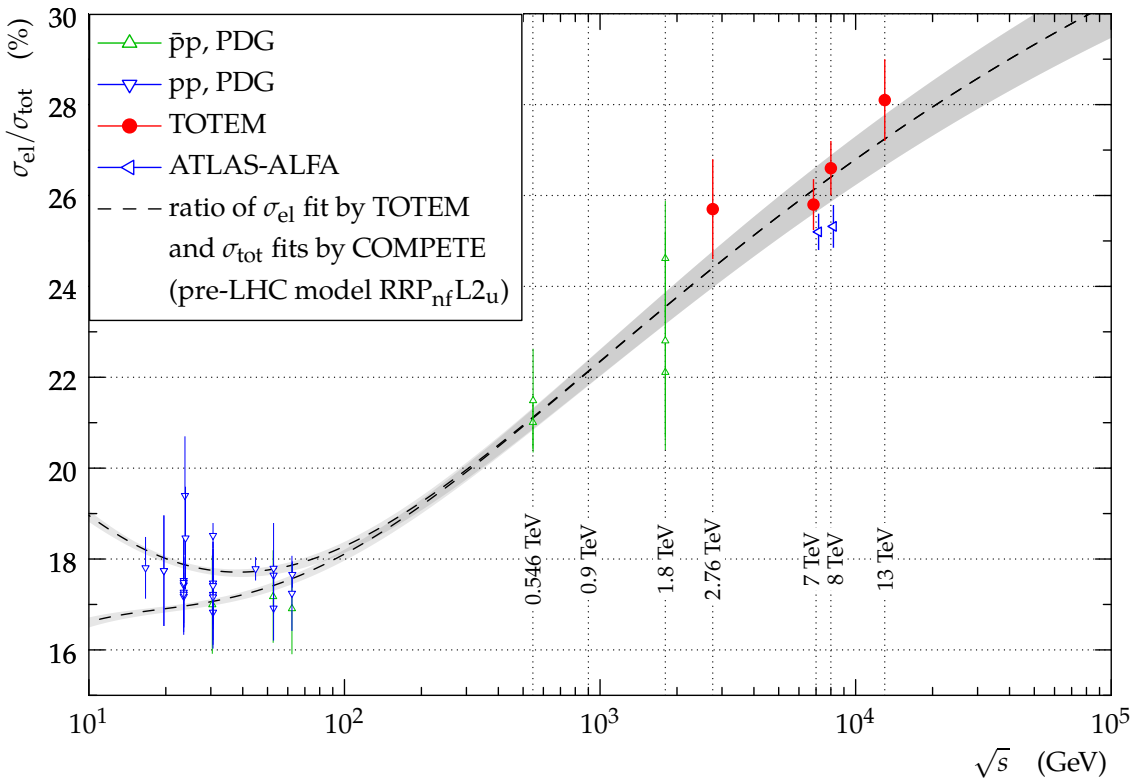
Fig. 6: (color). The elastic to total cross section ratio for pp and p\bar{p} collisions as a function of \sqrt{s} [1, 4–6, 22, 27, 28].
