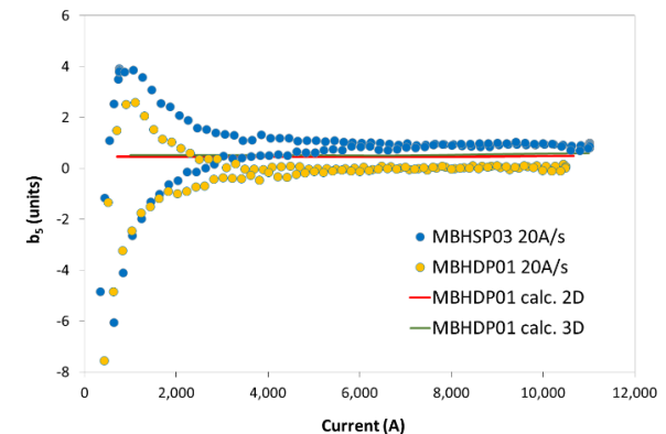
Figure 3: Normal quadrupole b_2 , sextupole b_3 , octupole b_4 and decapole b_5 vs. magnet current.
