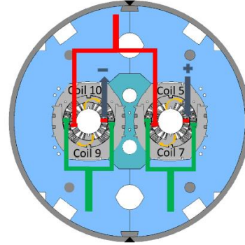
Figure 1: Coil layout and connection inside the yoke.
