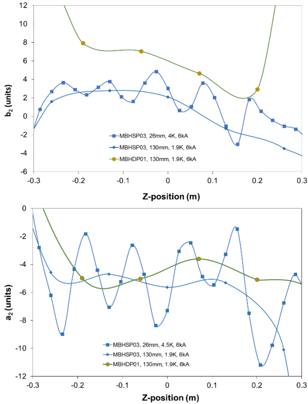
Figure 5: Variations of b_2 and a_2 along the magnet axis.
