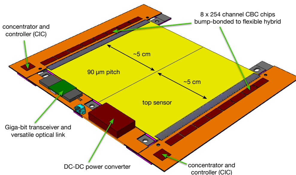
Figure 2. Conceptual view of the 2S-p_T module containing all electronic components. The sensors are planned to have an area of about 10 \times 10 \text{ cm}^2 with strips of about 5 cm length arranged in two rows (only the top sensor can be seen). The strip pitch is 90 \mu\text{m} . The two rows are read out from opposite ends via 2 \times 8 CBCs, bump bonded onto the top surface of the hybrid. The hybrid is folded around a stiffener and wire-bonded to both the top and the bottom sensor, bringing the signals from each sensor to the CBCs for amplification and correlation.
