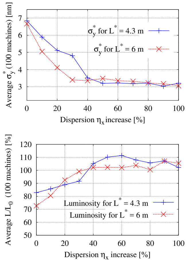
Figure 2: Average vertical beam size at the IP (top) and total luminosity, normalized to the design luminosity L_0 , (bottom) of 100 machines simulated after 1 iteration of BBA and linear knobs tuning of the FFS with increased dispersion level.
