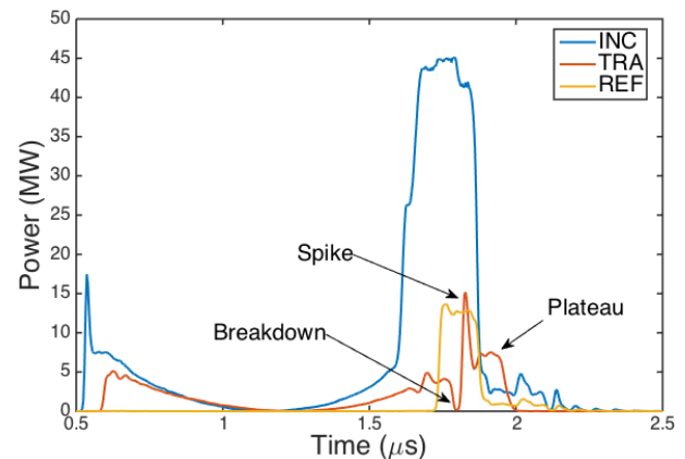
Figure 4: RF power signals in the case of a breakdown with beam. Incident (INC), transmitted (TRA) and reflected (REF) power signals are reported.
