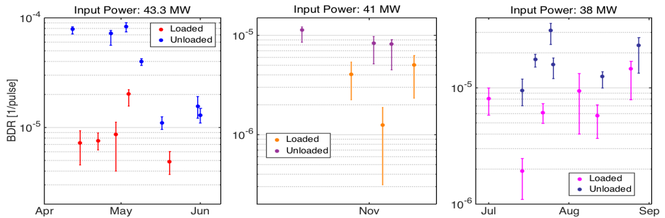
Figure 2: Measured BDR with alternating beam presence at different input power: 43.3 MW (left), 41 MW (center) and 38 MW (right).
