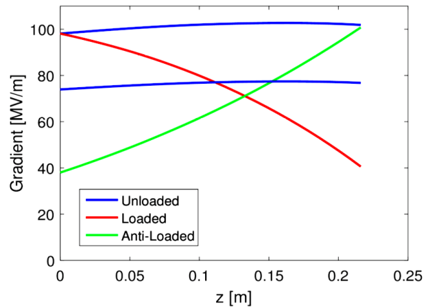
Figure 1: Longitudinal accelerating profile for the structure under test: unloaded (blue lines) 43.3 MW and 24.6 MW input power, loaded (red line) with 1.6 A of beam current and 43.3 MW input power, and anti-loaded (green line) with the same current and 6.5 MW input power.
