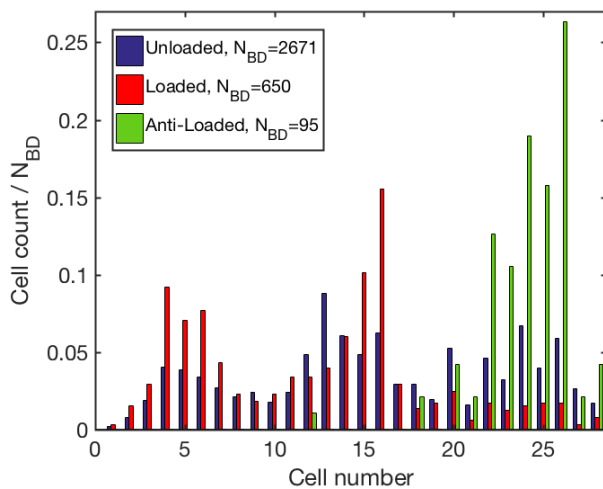
Figure 3: Breakdown distribution in the unloaded (blue), loaded (red) and antiloading (green).
