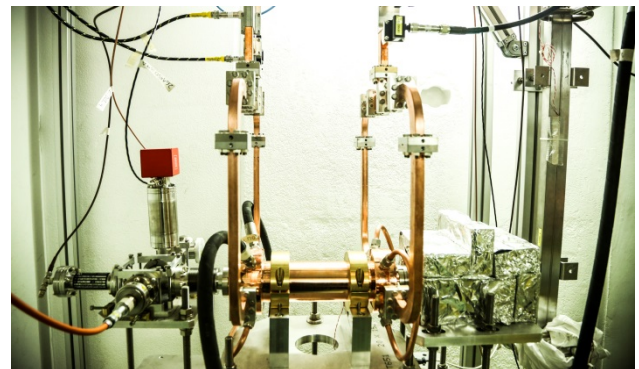
Figure 5: Structure installed in XBOX3.
