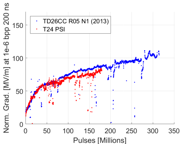
Figure 6: Structure conditioning history.
