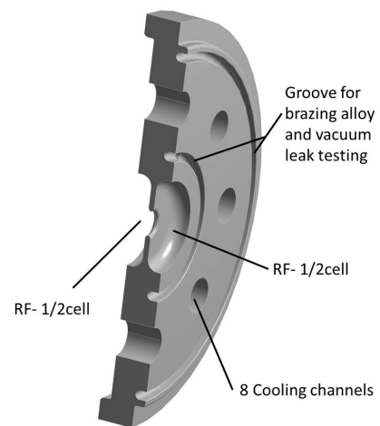
Figure 1: View of a section of one cell.
