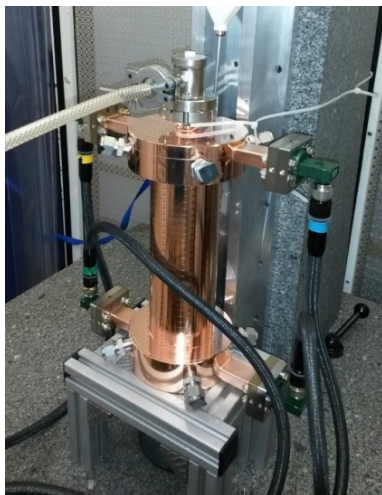
Figure 2: Structure ready for vertical bead-pulling.
