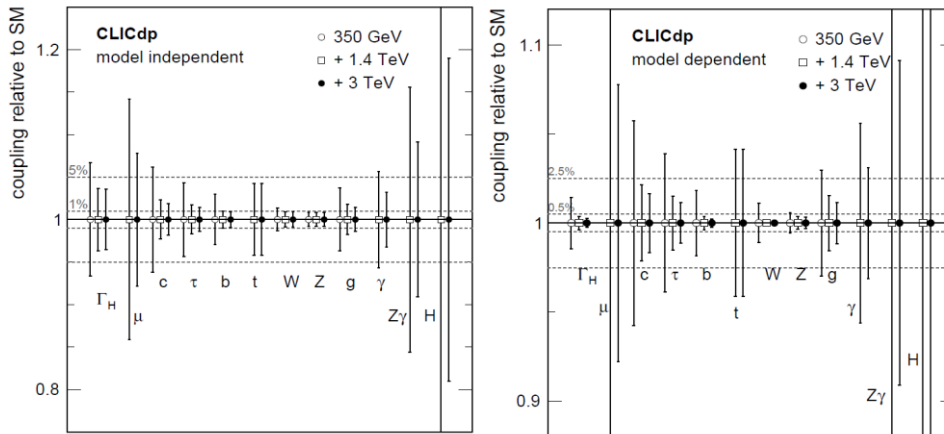
Figure 2. Illustration of the precision of the Higgs couplings and decay width of the studied three-stage CLIC programme [1]. Left: Results using a model-independent fit. Right: Results using a model-dependent fit.
